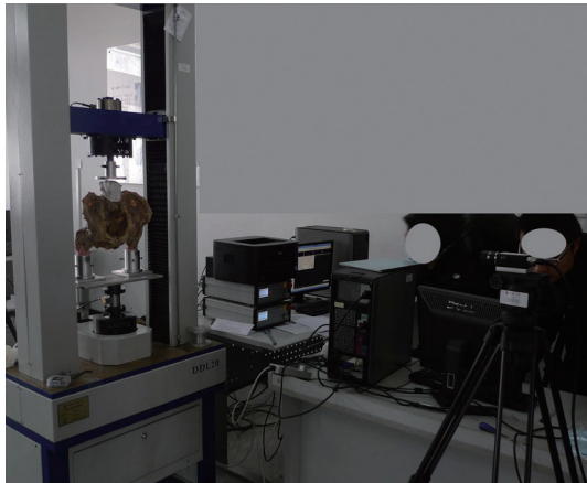
Figure 1 The setting of mechanical test.
