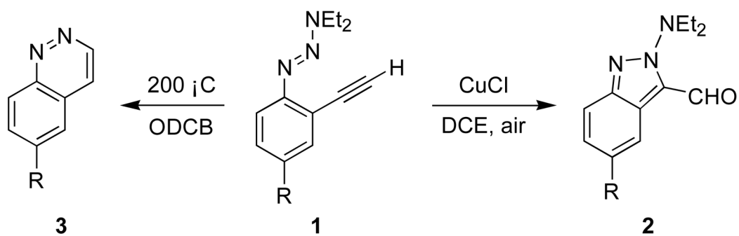
FIGURE 1. Dual cyclization pathways of azo-ene-yne 1 .
