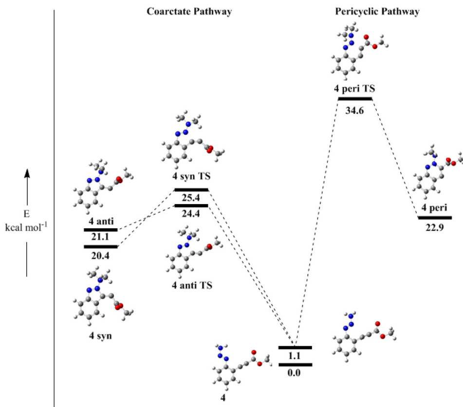
FIGURE 2. DFT (B3LYP/6-31G* + ZPE) calculated relative energies of reactants, transition states, and products for the cyclization of ester 4 to isoindazole carbenes and the cinnoline zwitterion.
