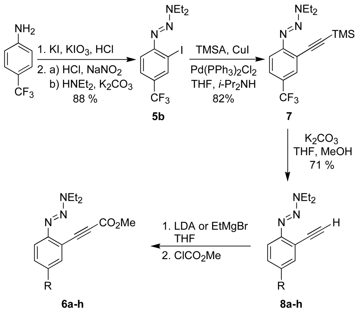
SCHEME 2. Synthesis of Azo-Ene-Yne 8b and Esters 6a-h
