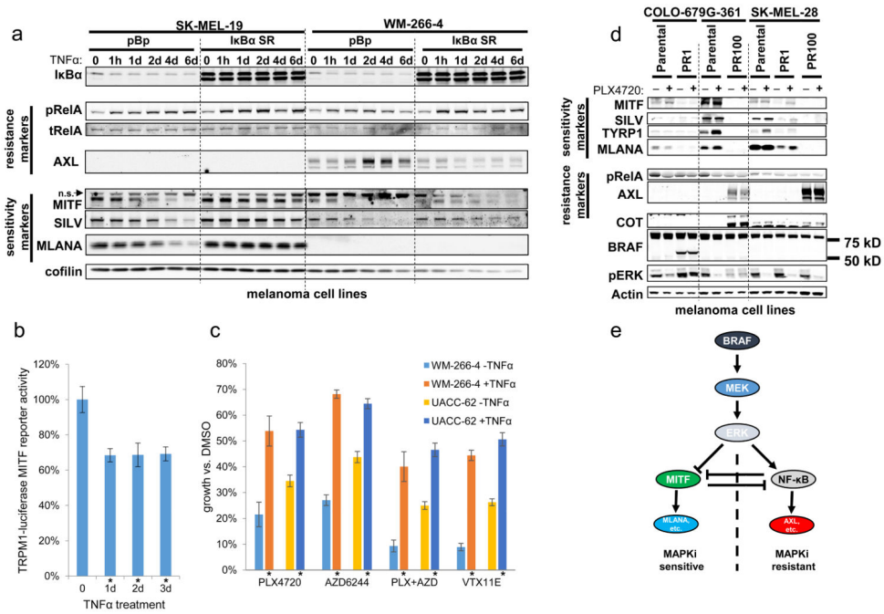
Figure 5. Plasticity of transcriptional class distinction in melanoma cell lines
