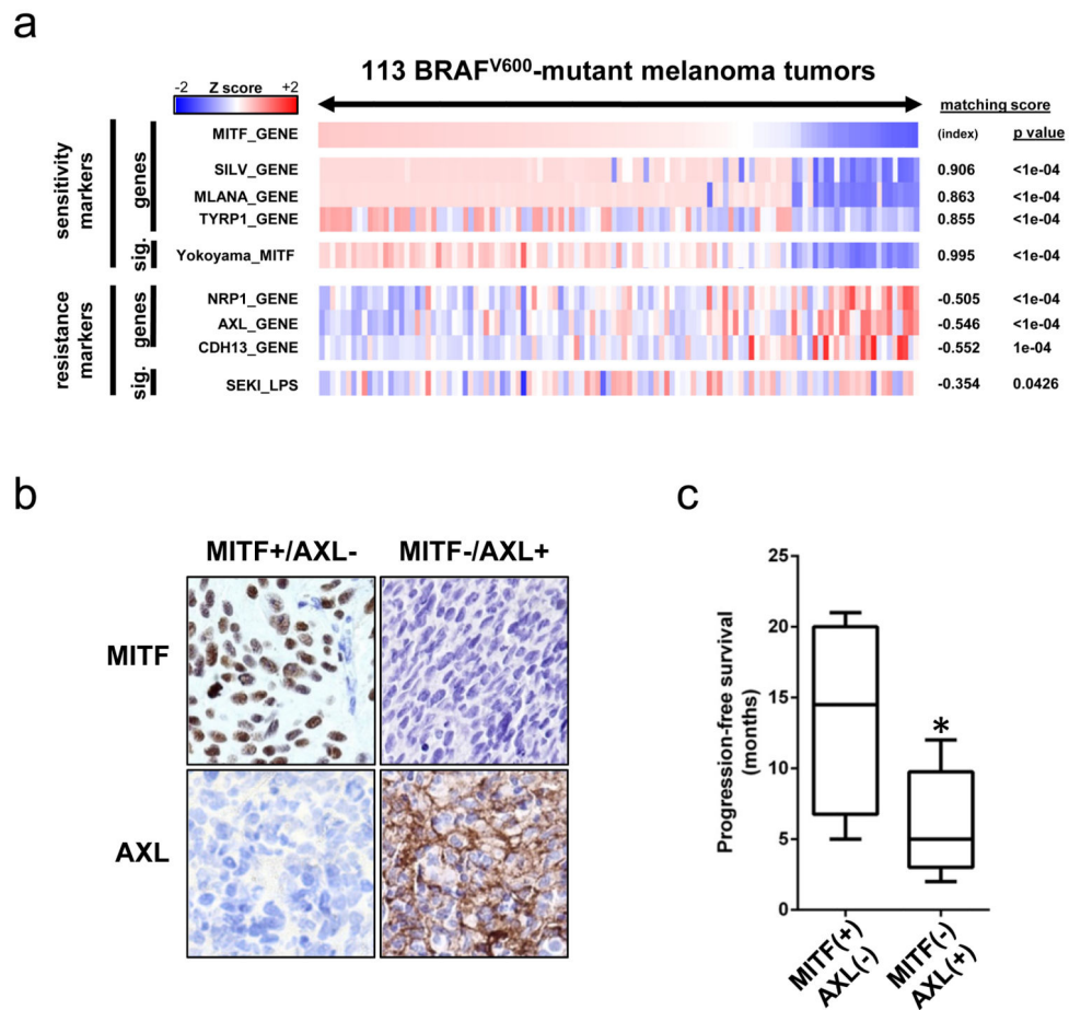
Figure 2. MITF-low/NF- \kappa B-high transcriptional class present and associated with resistance to MAPK pathway inhibition in human tumors
