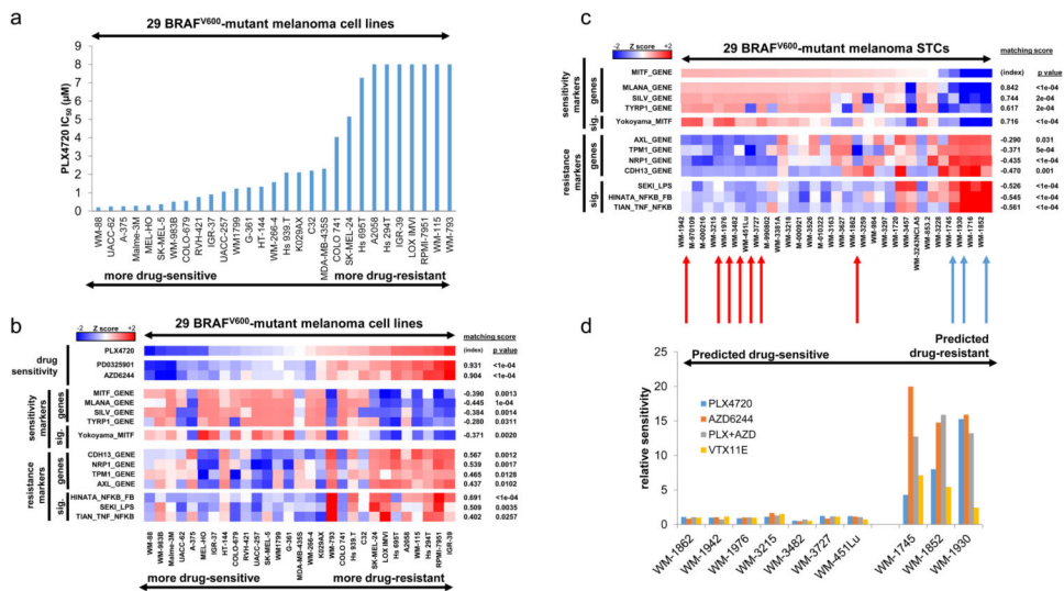
Figure 1. Association of expression classes with differential MAPK pathway inhibitor sensitivity in BRAF V600 -mutant melanoma in vitro (a) Sensitivity to PLX4720 (RAFi) across a collection of BRAF V600 -mutant melanoma cell lines. (b) Relationship between PLX4720 sensitivity and MITF-high versus NF-κB-high classes. (c) Transcriptional class distinction in BRAF V600 -mutant melanoma short-term cultures. (d) Relationship in short-term cultures between expression class and MAPK pathway inhibitor sensitivity. Graph shows GI 50 values relative to median GI 50 of the sensitive short-term cultures. PLX4720, RAFi; AZD6244, MEKi; VTX11E, ERKi.
