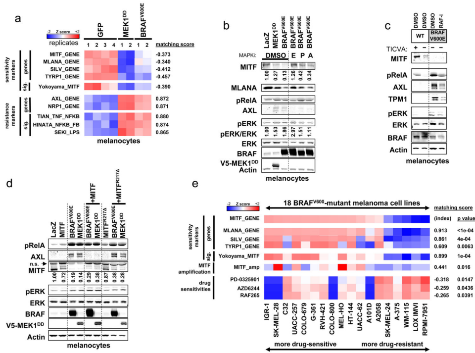
Figure 4. Establishment of transcriptional class distinction in melanocytes
