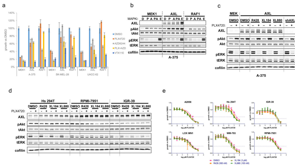
Figure 3. AXL is not necessary for maintenance of intrinsic resistance
