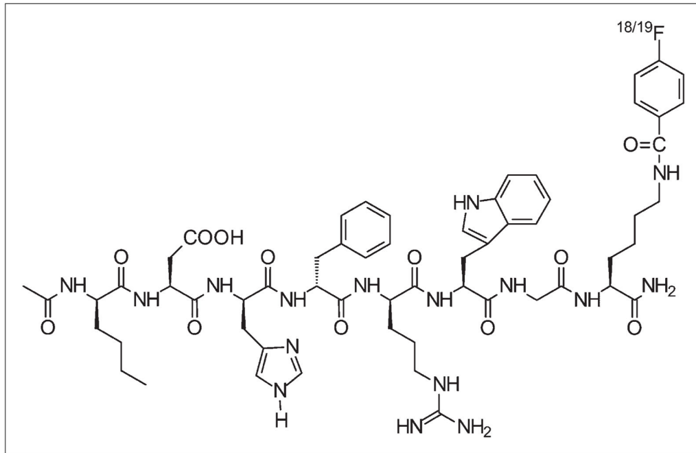
FIGURE 1. Schematic structure of ^{18/19}\text{F} -FB-NAPamide.
