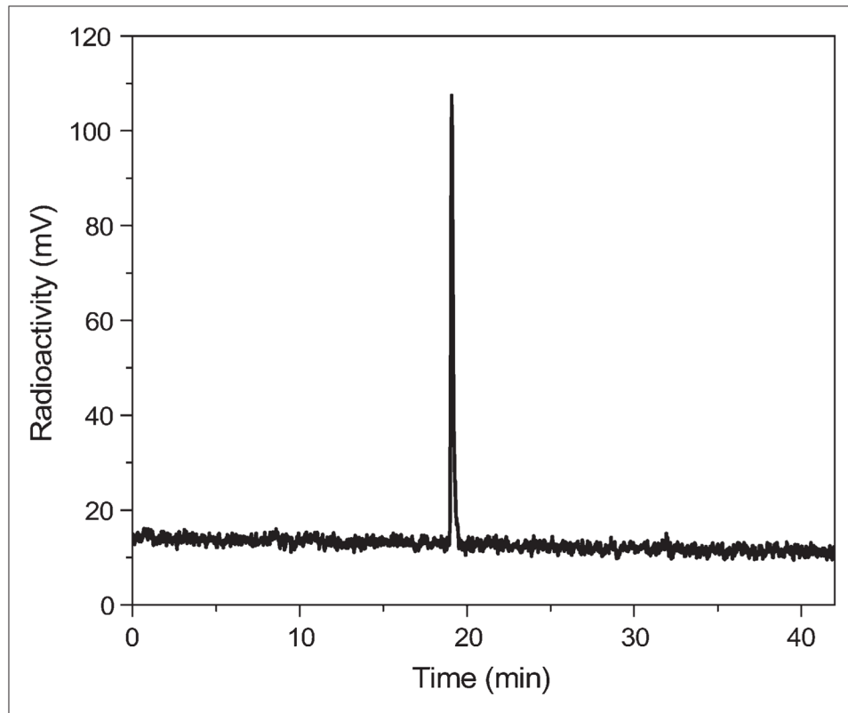
FIGURE 2. HPLC radiochromatogram of purified ^{18}\text{F} -FB-NAPamide.
