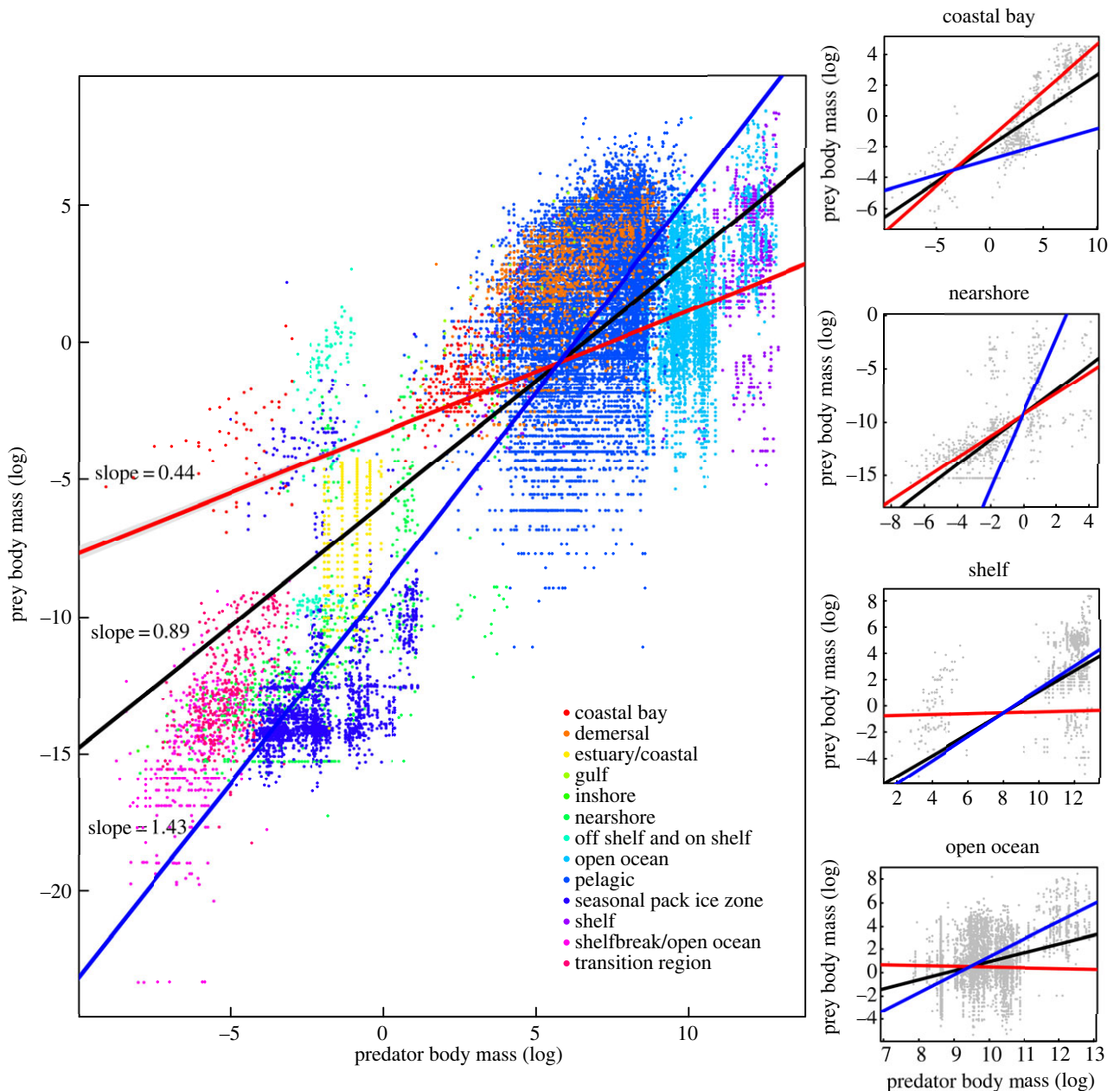
Figure 1. Left: prey body size (log) against predator body size (log) across marine habitats. Red ( T = 29^{\circ}\text{C} ), black ( T = 15^{\circ}\text{C} ) and blue lines ( T = -1.3^{\circ}\text{C} ) represent predicted curves from the best model. 95% confidence intervals are displayed in grey. Right: same as in left for a subset of the habitats studied (coastal bay is not significant). (Online version in colour.)
