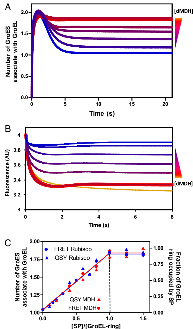
Fig. 2. The football complex encapsulates two misfolded proteins simultaneously. (A) Pre-steady-state formation of GroEL:GroES 2 monitored by FRET. Concentrations of dMDH are indicated as follows (from top to bottom): 0.43, 0.357, 0.286, 0.229, 0.171, 0.114, 0.057, and 0 \mu\text{M} ; 2 \mu\text{M} GroEL IAEDANS subunit (0.3- \mu\text{M} rings), 4 \mu\text{M} GroES F5M subunit, and 0.5 mM ATP were used for all of the measurements. The reactions were initiated by introducing ATP+GroES F5M into solution containing GroEL IAEDANS preincubated with dMDH. The summary plot of this set of experiment is shown in C as a red circle. (B) Encapsulation of dMDH by GroEL:GroES 2 shown by titrating GroEL ring with dMDH QSY7 reported by the quenching of F5M labeled GroES. The experiments were performed under the same condition as those in A. The bottom yellow trace was generated by also including 1 mM BeCl 2 and 10 mM NaF to restrict the measurement to single turnover condition and was used as 100% SP occupation level. The summary plot of this set of experiment is shown in C as red triangles. (C) Determination of SP (dMDH in red and dRubisco in blue) encapsulation stoichiometry by the GroEL:GroES 2 complex. Two different ways are used: (i) the FRET signal between GroEL IAEDANS and GroES F5M using unlabeled SPs (circles) (primary data of dMDH shown in A and that of dRubisco shown in Fig.S1B) and (ii) quenching of GroES F5M by SP QSY7 upon SP encapsulation and formation of the GroEL:SP 2 :GroES 2 complex (triangles) (primary data of dMDH shown in B and that of dRubisco in Fig. S1C).
