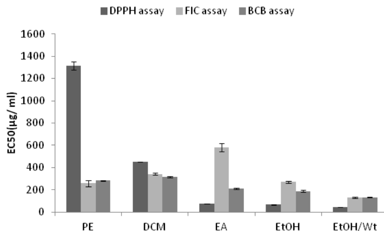
Figure 1. Antioxidant activity of A. biennis extracts from petroleum ether (PE), dichloromethane (DCM), ethyl acetate (EA), ethanol (EtOH) and ethanol/water (EtOH/Wt).
