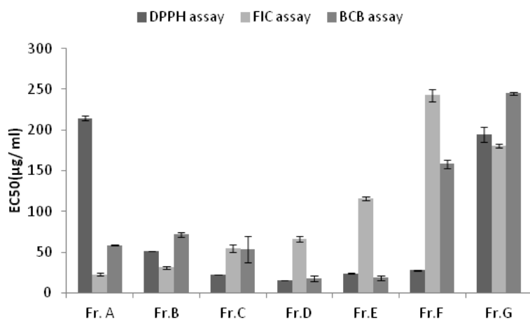
Figure 2. Antioxidant activity of different fractions from hydroethanolic extract of A. biennis .
