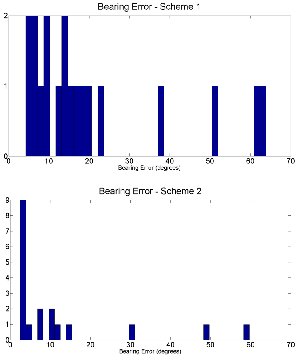
Figure 7. Histograms of the absolute value of bearing estimation error, shown for Scheme 1 (top) and Scheme 2 (bottom). Note that the error is lower for Scheme 2 than for Scheme 1.
