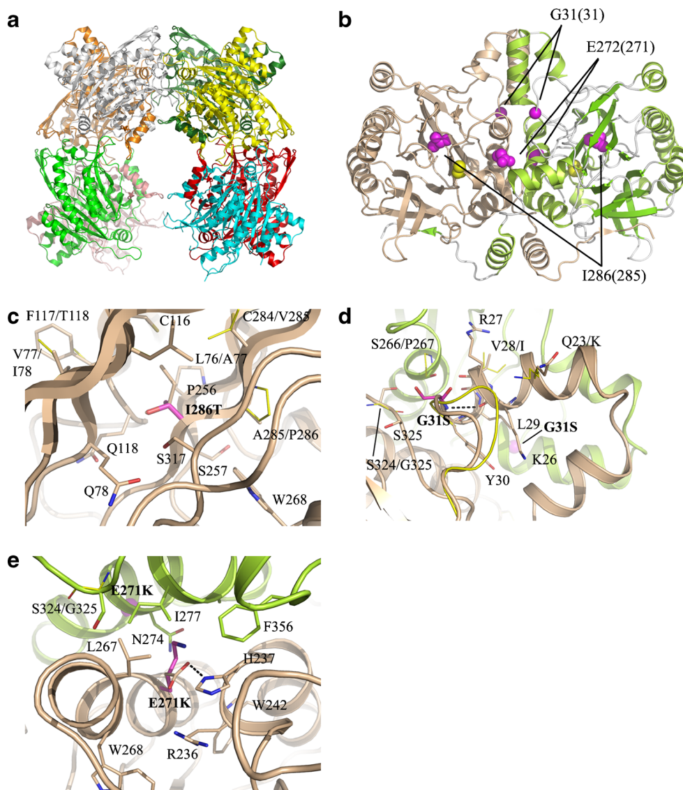
Fig. 1 DmβUP crystal structure and mutation site environment in the homology model of human βUP. (a) Schematic view of homooctameric DmβUP with each subunit coloured differently. (b) Schematic view of a dimeric unit of DmβUP. For one of the subunits, β-strands are depicted in green, helices in yellow-green and loops in white, with the other subunit coloured salmon. Mutation sites are highlighted by space-filling models of the respective amino acid side chains in magenta. Labels first list the corresponding site in DmβUP. Location of the active site is indicated by space-filling models of the active site cysteine (C233 in human βUP, C234 in DmβUP) in yellow. (c–e) Enlarged views of I286T, G31S and E271K mutation sites. The homology model of human βUP is shown with different colours (salmon and green) for two separate subunits. Additional subunits were omitted as none of the mutations occur near
