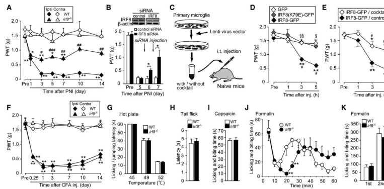
Figure 4. Microglial IRF8 Is Necessary for Abnormal Pain Hypersensitivity Caused by PNI (A) PWT of Irif8 -/- and WT mice before (Pre) and after PNI (n = 4; *p < 0.05, **p < 0.01 versus Pre; #p < 0.05, ##p < 0.01, ###p < 0.001 versus the ipsilateral side of WT mice). C, contralateral; I, ipsilateral. (B) Reversal of PNI-induced allodynia by intrathecal administration of IRF8 siRNA (20 pmol) once a day for 2 days (on 5 and 6 days post-PNI) in WT mice (n = 3–6, *p < 0.05). Upper, representative immunoblots of IRF8 and β-actin proteins in the spinal cords of mice treated with control and IRF8 siRNAs on day 7 post-PNI. (C) Experimental protocol. (D) PWT of WT mice intrathecally administered with cultured microglia overexpressing either GFP, IRF8–GFP or IRF8(K79E)–GFP (n = 5–6, **p < 0.01 versus Pre; #p < 0.05 versus WT mice with GFP microglia; §p < 0.05, §§p < 0.01 versus WT mice with IRF8–GFP microglia). (E) Allodynia by IRF8-transduced cultured microglia was prevented by preincubating microglia with a cocktail of IL-1β neutralizing antibody (5 μg) and CatS inhibitor (5 pmol) for 15 min before the intrathecal injection of microglia (n = 6–7, *p < 0.05, **p < 0.01 versus Pre; #p < 0.05, ###p < 0.001 versus IRF8–GFP/ control group). (F) PWT of WT and Irif8 -/- mice before (Pre) and after intraplantar CFA injection (n = 5, **p < 0.01 versus Pre). (G) Hot-plate test. Values represent the latency (s) for animals to lick their hindpaws or jump (n = 6). (H) Tail-flick test. Values represent the latency (s) to flick their tail from the heat source (n = 4). (I–K) Capsaicin (I) and formalin (J and K) test. Values are the duration (s) of nociceptive behaviors (I: n = 6, J: n = 8) (**p < 0.01 versus WT mice). (K) Total duration (s) of nociceptive behaviors for 0–5 min (first phase) and for 10–60 min (second phase). Values are the mean ± SEM for all groups. See also Figure S4.
