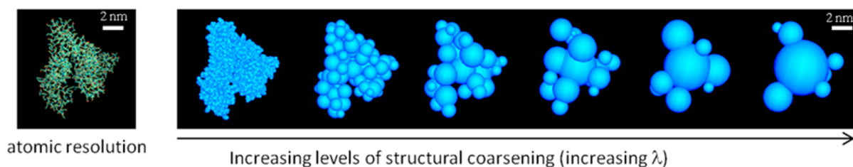
Figure 1. Structural coarse-graining of albumin (based on PDB: 1AO6). Reverse coarsening (fine graining) to any \lambda level is straightforward (used in Figures 6–8). The hydrodynamic radius R_H of albumin in water has been measured at \sim 3.2 – 3.48 nm. 22,44 For the rigid model used here, n = 7 and \rho_i = R_i + d_w , where d_w is the average thickness of the hydration layer surrounding the protein. Using a single layer ( d_w = 2.8 Å), eq 6 yields R_H = 3.33 nm. The calculated translational and rotational diffusion constants are D_T \sim 6.6 \times 10^{11} m 2 s -1 and D_R \sim 4.4 \times 10^6 s -1 , respectively, close to the experimental values. 21 The rotational correlation times \tau_D^{(1)} and \tau_D^{(2)} (Debye's relaxation time) of the albumin macrodipole ( \sim 500 D 21 ) are thus \sim 33 ns and \sim 0.1 \mu s, respectively. The model can be used to calculate dielectric and spectroscopic properties of albumin solutions, although the relaxation times indicate that long dynamics simulations would be needed to properly sample the conformational space, which justifies the choice of Monte Carlo sampling used in this study.
