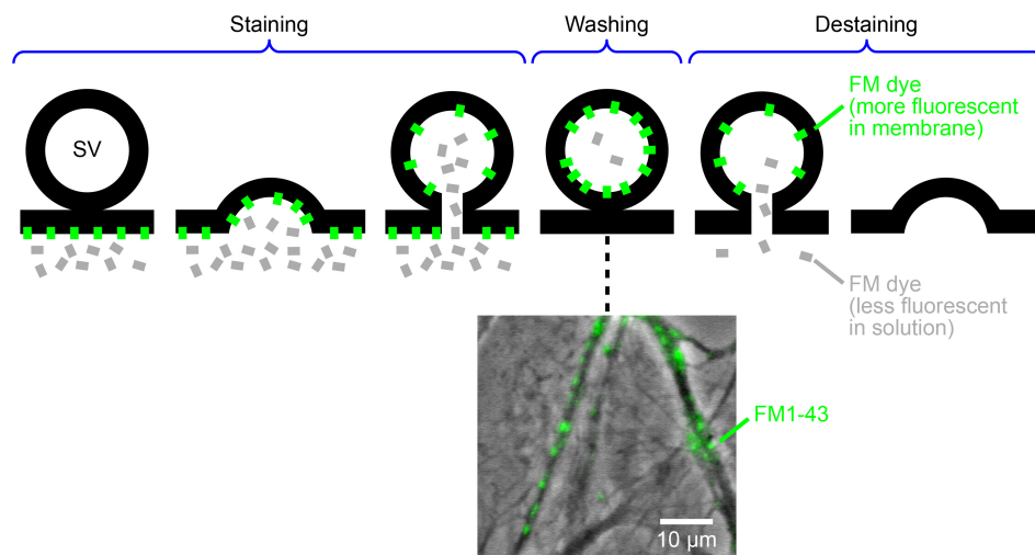
Figure 2. Basic scheme of FM dye usage. After application to neurons, the FM dye inserted into the plasma membrane becomes fluorescent (green), whereas that in the aqueous solution is much less fluorescent (gray). A synaptic vesicle (SV) is loaded (stained) by the FM dye, when it undergoes endocytosis, typically following exocytosis. Washing out the FM dye in extracellular solution enables only the stained vesicles to be fluorescent. Subsequently, a synaptic vesicle is unloaded (destained) when it undergoes exocytosis and therefore releases the FM dye. An image below illustrates an exemplar staining of cultured hippocampal neurons with FM1-43 (an overlay of fluorescence and phase contrast images). It is of note that, in the protocol described in this paper, the fluorescent puncta represent presynaptic nerve terminals (diameters ~1 μm in typical central neurons) with clusters of stained synaptic vesicles, not the individual synaptic vesicles (diameters ~40 nm). For simplicity, this scheme represents a general idea of exo-endocytosis of synaptic vesicles. It can include multiple forms of exo-endocytosis, such as the full-collapse fusion followed by clathrin-mediated endocytosis, the transient kiss-and-run exo-endocytosis, and the bulk endocytosis 64 . Please click here to view a larger version of this figure.
