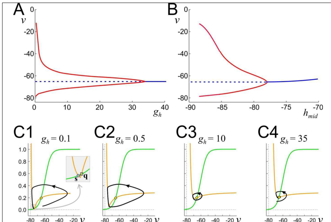
Figure 6. Bifurcation diagrams and phase plane behaviors for system (4) and v_{\text{cutoff}} = E_{\text{NL}} A: Bifurcation diagram with g_h as parameter. Solid (dashed) lines/curves indicate stable (unstable) fixed points (blue)/periodic orbits (red). B: Bifurcation diagram with h_{mid} as parameter and g_h = 1 \mu\text{S} . C1-C4: Phase planes and limit cycles for various values of g_h as noted. v in mV, g_h in \mu\text{S} . Inset in C1 highlights the fixed points q and s .
