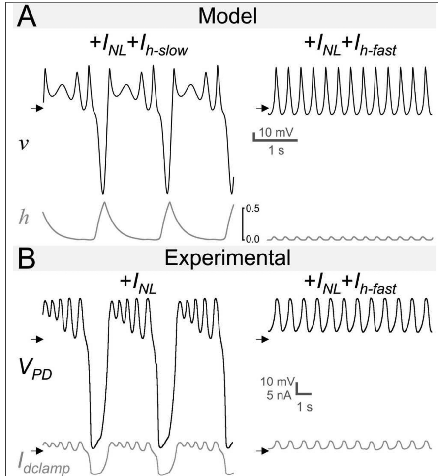
Figure 8. Hyperpolarizing dips in system (3) and experimental verification
