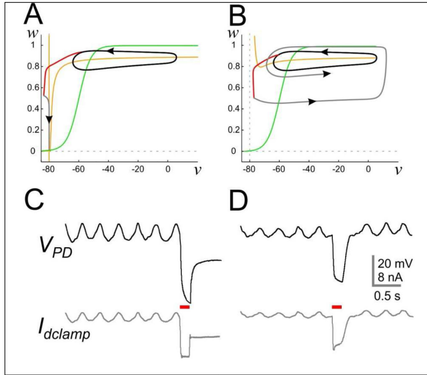
Figure 7. Perturbation of the periodic orbit of system (4) without and with I_h A. When g_h = 0 , perturbation (red) of the trajectory along a stable periodic orbit (black) by injecting a hyperpolarizing current pulse causes the trajectory (gray) to converge to the stable fixed point at v = E_K . B. When g_h > 0 , the same type of perturbation cannot remove the trajectory from the basin of attraction of the periodic orbit and the ensuing trajectory (gray) is attracted back to the periodic orbit. C. and D. Corresponding voltage traces from a biological PD neuron with I_{NL} injected using dynamic clamp (and v_{cutoff} = E_{NL} ). A -5 nA current pulse (red bar) shuts down the oscillations in the absence of I_h ( C ). In the presence of a dynamic-clamp injected instantaneous I_h , the same current pulse only provides a brief interruption in the oscillations ( D ).
