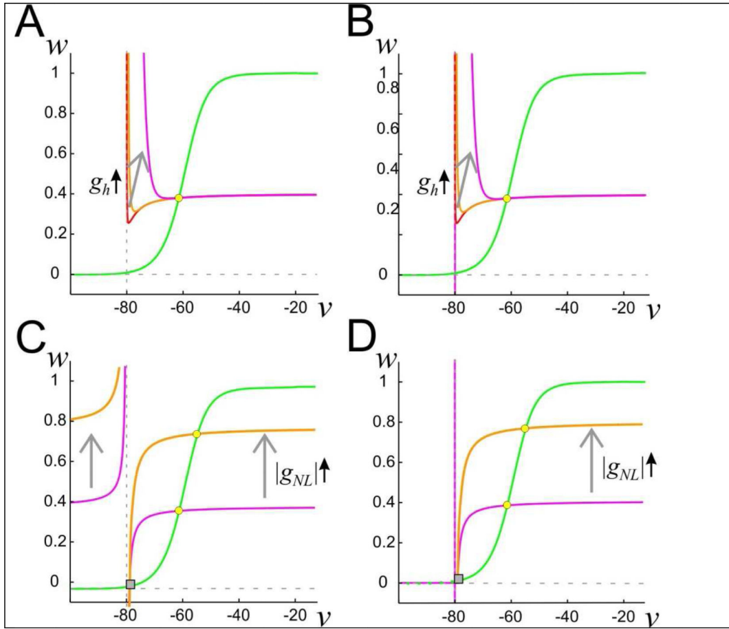
Figure 1. Phase plane structure of the linear negative conductance-based neuron model
