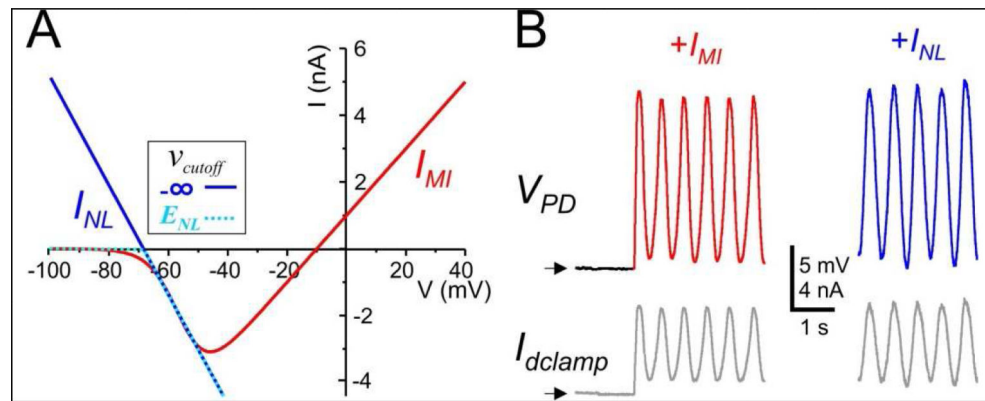
Figure 2. Linear negative conductance current elicits oscillations in PD neurons
