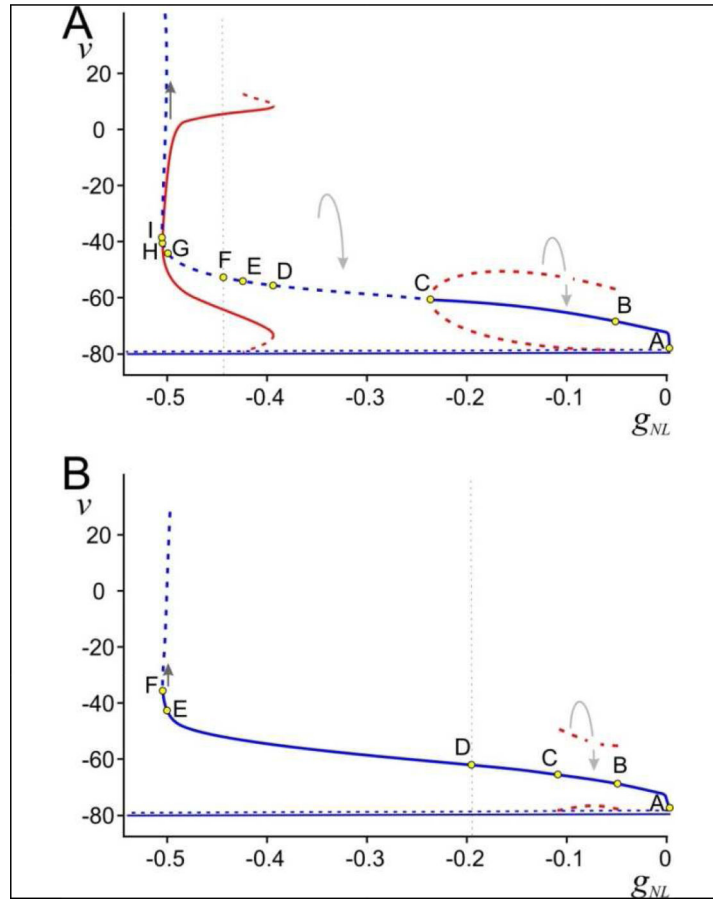
Figure 5. Alternative bifurcation diagrams for system (6)
