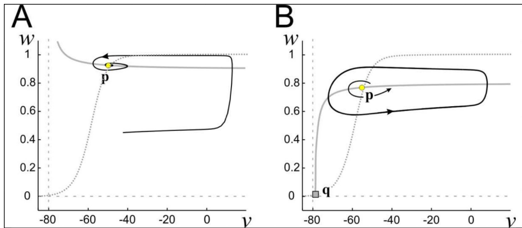
Figure 3. Phase plane of the simplified linear negative conductance current model
