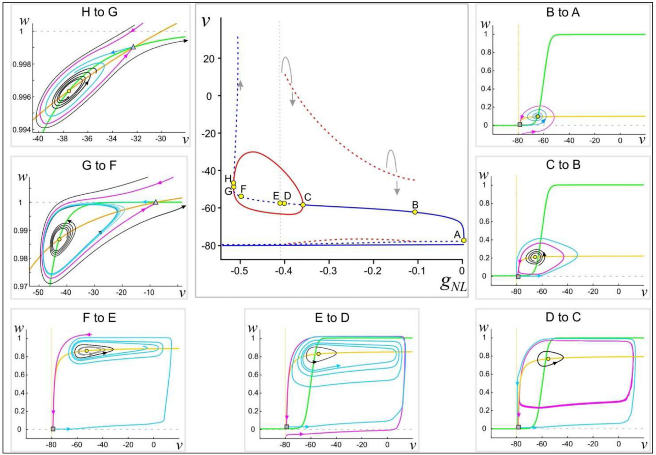
Figure 4. Bifurcation diagrams for system (6) and associated phase planes
