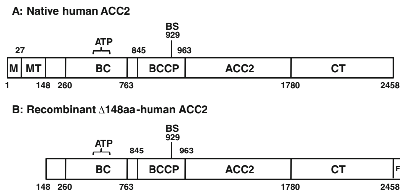
Fig. 1 A schematic presentation of human ACC2 domains. a Native hACC2. ACC2, human acetyl-CoA carboxylase 2; ATP, ATP-grasp domain; BC, biotin carboxylase domain; BCCP, biotin carboxyl carrier protein domain; BS, biotinylation site; CT, carboxyltransferase domain;
