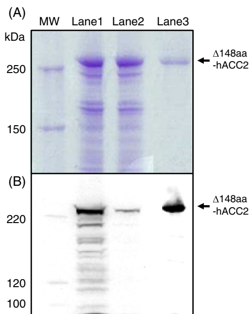
Fig. 2 The expression of recombinant \Delta 148\text{aa-hACC2} was confirmed by analysis of SDS-PAGE (a) and Western blot (b). MW , molecular weight markers; Lane 1 , protein extracts after infection; Lane 2 , flow through during FLAG-tag purification; Lane 3 , purified and concentrated \Delta 148\text{aa-hACC2} . An anti-FLAG M2 antibody and an anti-mouse IgG-HRP were used to detect purified \Delta 148\text{aa-hACC2}
