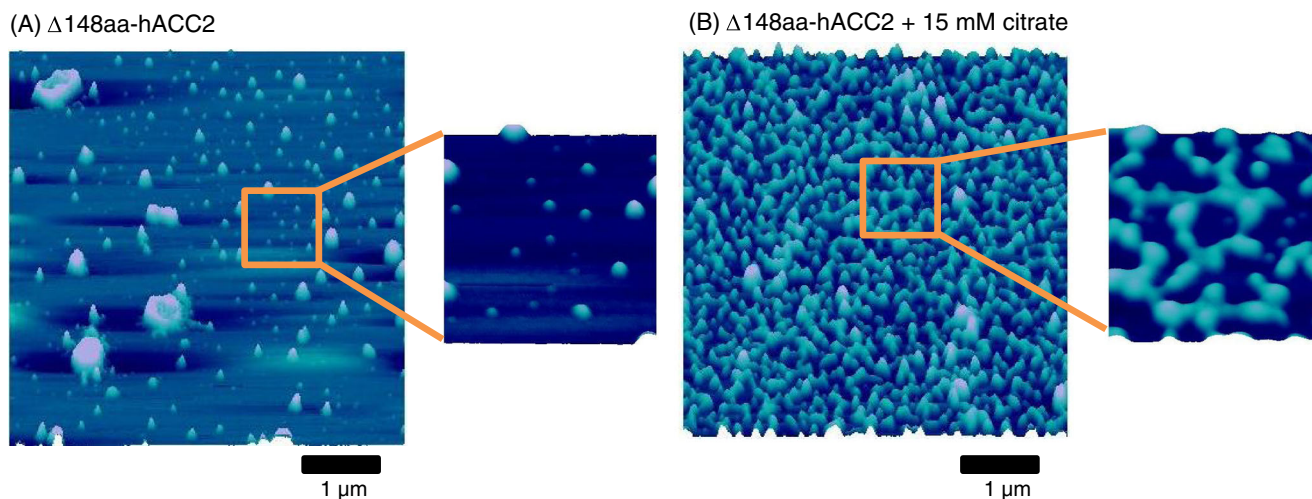
Fig. 6 Atomic force microscopy nanoscale images of \Delta 148\text{aa-hACC2} . a \Delta 148\text{aa-hACC2} alone. b \Delta 148\text{aa-hACC2} with 15 mM citrate after 20-min incubation at 37 °C. Citrate induced the filaments formation
