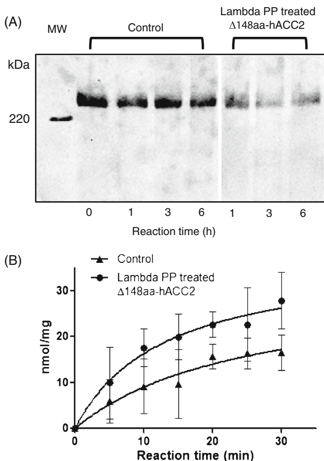
Fig. 4 Dephosphorylation of purified \Delta 148\text{aa-hACC2} influences catalytic function. a Dephosphorylation of \Delta 148\text{aa-hACC2} treated with Lambda PP was assessed by Western blotting using a monoclonal anti-phosphoserine antibody produced in mouse and an anti-mouse IgG-HRP. b Lambda PP treated \Delta 148\text{aa-hACC2} enhanced catalytic activity
