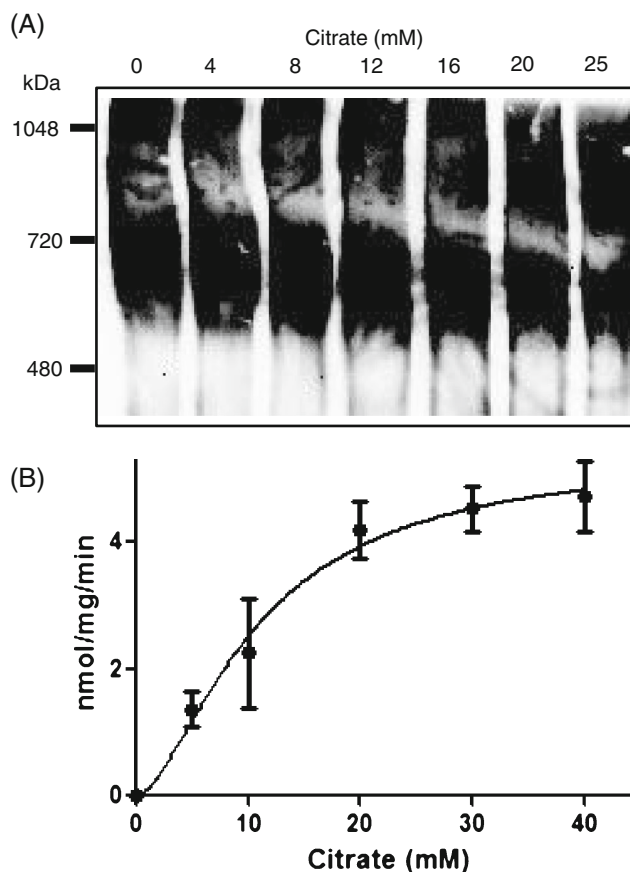
Fig. 5 Polymerization and enzyme activities of \Delta 148\text{aa-hACC2} were modulated by citrate concentration. a Degree of polymerization of \Delta 148\text{aa-hACC2} by different concentration of citrate (0, 4, 8, 12, 16, 20, and 25 mM). The polymerization was confirmed using Native-PAGE. b Enzymatic activities by citrate concentration. All data are means \pm S.D. from three separate experiments
