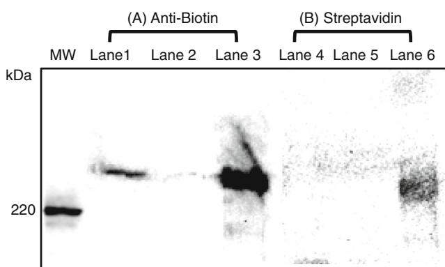
Fig. 3 The purified \Delta 148\text{aa-hACC2} possesses posttranslational biotinylation confirmed by Western blot analysis using an anti-biotin antibody (A) and streptavidin HRP conjugate (B). MW , molecular weight markers; Lanes 1 and 4 , protein extracts after infection; Lanes 2 and 5 , flow through during FLAG-tag purification; Lanes 3 and 6 , purified and concentrated \Delta 148\text{aa-hACC2} . An anti-biotin antibody and a streptavidin HRP conjugate were used as primary antibodies. A rabbit anti-goat IgG-HRP and an anti-mouse IgG-HRP were used as secondary antibodies
