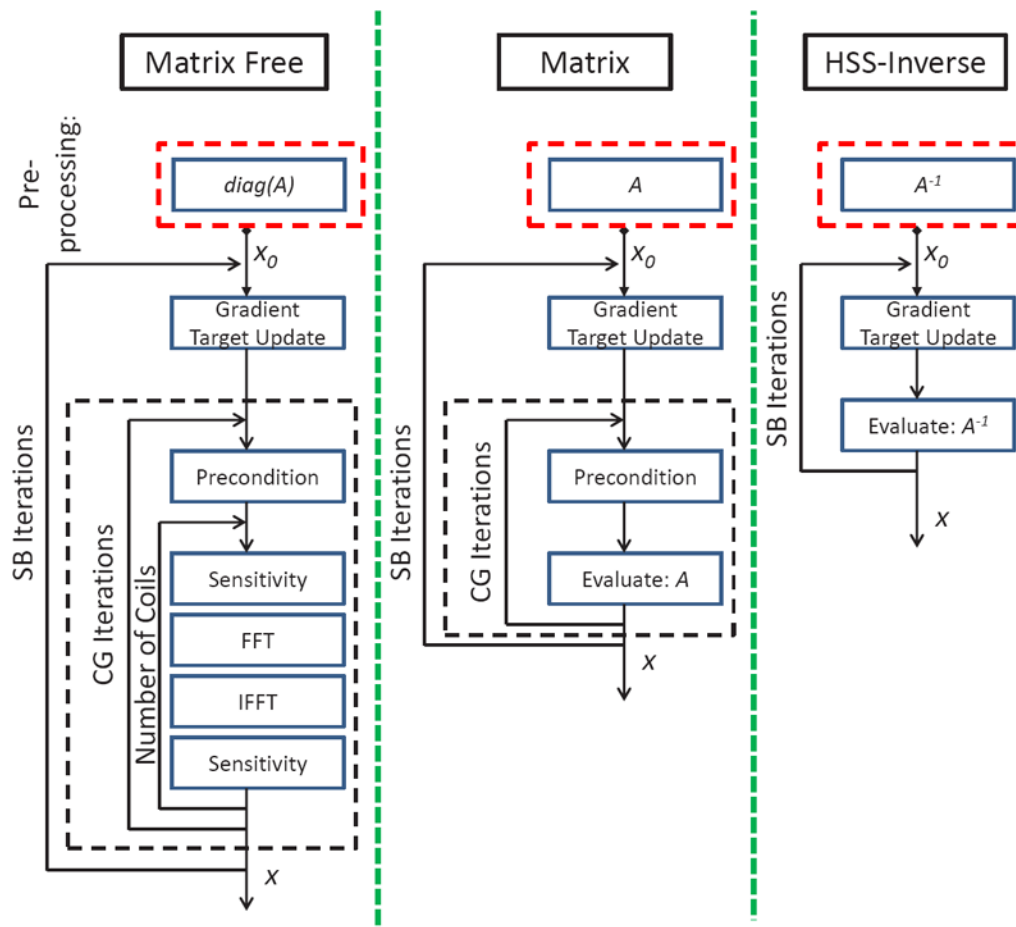
Figure 1. Split Bregman CS+SENSE implementations are illustrated. The required pre-computation is shown above the corresponding flow diagrams. The Matrix Free and Matrix methods rely on iterative CG solutions, while the HSS-Inverse method gives a direct solution for each Split Bregman iteration. The CG based approaches are optimized with the diagonal Jacobi pre-conditioner.
