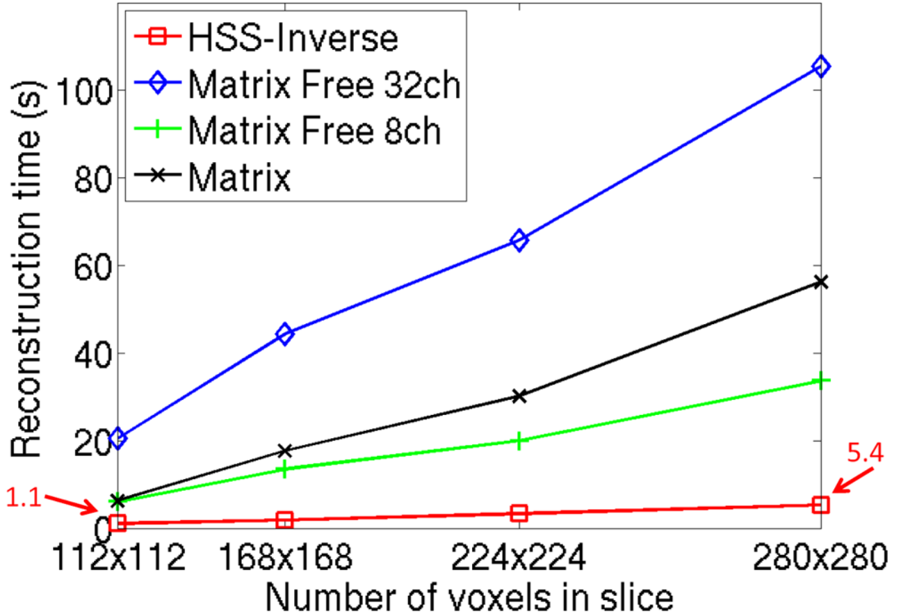
Figure 5. Computational scaling with respect to image size for CG and HSS based reconstruction methods, see Figure 1 for algorithm flow-diagrams. R = 3 acceleration is applied to the T2 weighted images. A 10^{-6} tolerance is assumed for all algorithms to ensure consistent final image error. All methods include 5 iterations of Split Bregman with a TV weighting \beta = 3 \cdot 10^{-3} and soft-thresholding \epsilon = 2 \cdot 10^{-1} . The Jacobi pre-conditioner is used for all CG methods. The use of Cartesian optimized coil compression from 32 to 8-channels is explored for the Matrix Free method. The smallest and largest reconstruction times for HSS-Inverse are identified with arrows.
