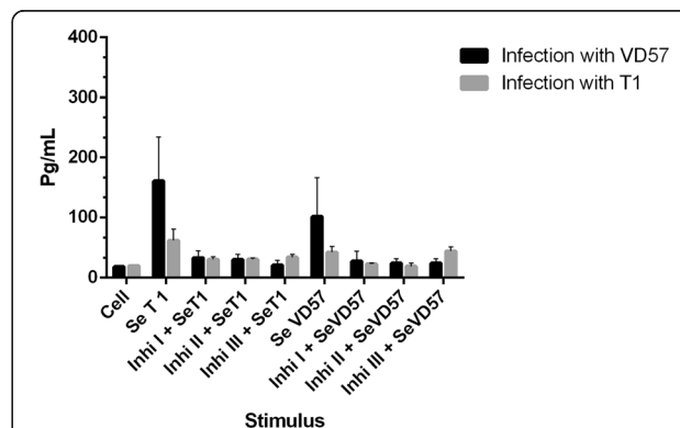
Figure 2 Effect of MAPK pathway inhibitors MAPK p38 (Ini I), ERK 1 / 2 (Ini II) and ERK 2 (Ini III) on the production of TNF- \alpha by splenic cells obtained from CBA mice after 60 days of infection with virulent (VD57) and attenuated (T1) C. pseudotuberculosis strains, under stimulation by secreted/excreted antigens (SeT1 and SeVD57). Each experiment was carried out \geq 3 times in triplicate. * p < 0.05 with respect to stimulation by SeT1; # p < 0.05 with respect to stimulation by SeVD57.
