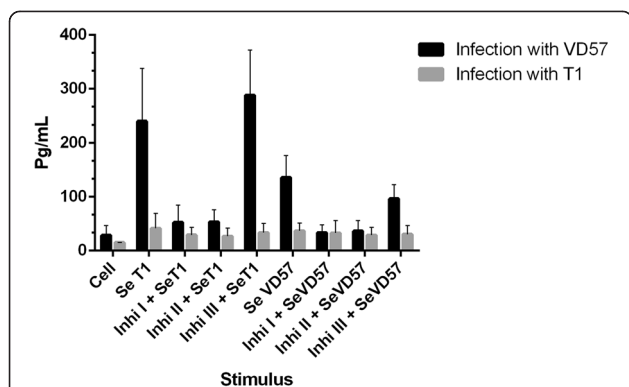
Figure 1 Effect of MAPK pathway inhibitors MAPK p38 (Ini I), ERK 1 / 2 (Ini II) and ERK 2 (Ini III) on the production of TNF- \alpha by splenic cells obtained from CBA mice after 30 days of infection with virulent (VD57) and attenuated (T1) C. pseudotuberculosis strains, under stimulation by secreted/excreted antigens (SeT1 and SeVD57). Each experiment was carried out \geq 3 times in triplicate. * p < 0.05 with respect to stimulation by SeT1; # p < 0.05 with respect to stimulation by SeVD57.
