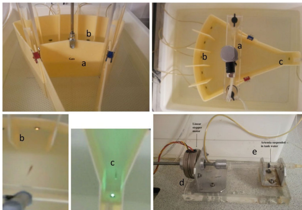
Fig. 1. Testing environment used to train zebrafish on 5-CSRTT.
