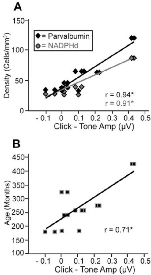
Figure 11. Amplitude differences as a function of cell density and age. The difference between threshold amplitudes of clicks and high-frequency tone auditory brainstem responses as a function of cell density (A) and age (B). Higher values indicate greater prominence of click amplitudes over tones amplitudes at threshold. Again, this suggests that clicks and tones are processed differently and that the magnitude of this difference correlates with both cell density and age. Note that the x-axis is identical in both panels for direct comparison.
