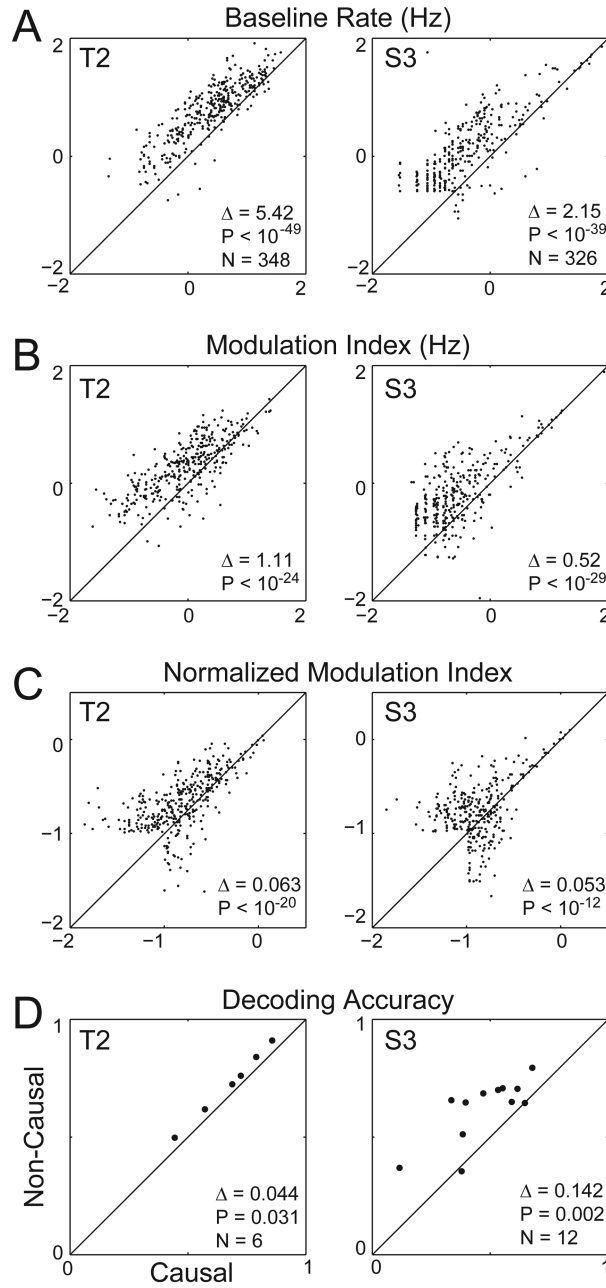
Figure 2. Comparing tuning metrics between causal and non-causal threshold crossing events. (A) Scatter plot of baseline threshold crossing rates using the causal filter method (x-axis) versus baseline threshold crossing rates using the non-causal filter method, plotted on a log scale, for T2 (left column) and S3 (right column). \Delta gives the mean difference in the baseline rates between the causal and non-causal filter methods. (B) Same as (A), except plotting modulation depth. (C) Same as (A), except plotting normalized modulation depths. (D) The decoding accuracy (defined as the mean dot product between the decoded and actual cursor direction) for the six T2 sessions (left column) and the twelve S3 sessions (right column).
