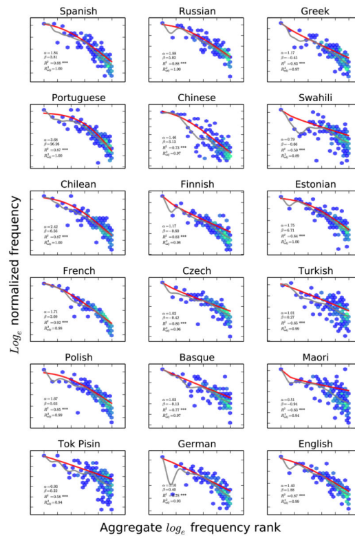
Fig. 2. Cross-linguistic word frequency distributions using words from a Swadesh list (data provided by Calude & Pagel, 2011). Here, the x -location of each point (word) is fixed across languages according to the aggregate frequency rank of the word's meaning on an independent set of data. The systematicity here means that the word frequency distribution falls off similarly according to word meaning across languages and approximately according to a power law like Eq. 2 (red)
