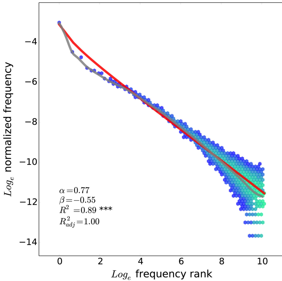
Fig. 9. Frequency distribution of the 25,000 most frequent “words” in the ANC, where “e” rather than space (“ ”) was treated as a word boundary. This exhibits a clear near-Zipfian distribution, with the frequency of these words falling off much like Eq. 2
