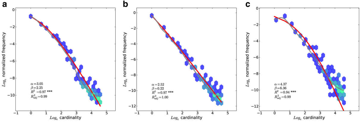
Fig. 3. Power law frequencies for number words (“one,” “two,” “three,” etc.) in English (a), Russian (b), and Italian (c), using data from Google (Lin et al., 2012). Note that here the x -axis is ordered by cardinality, not frequency rank, although these two coincide. Additionally, decades (“ten,” “twenty,” “thirty,” etc.) were removed from this analysis due to unusually high frequency from their approximate usage. Here and in all plots, the red line is the fit of Eq. 2, and the grey line is a LOESS
