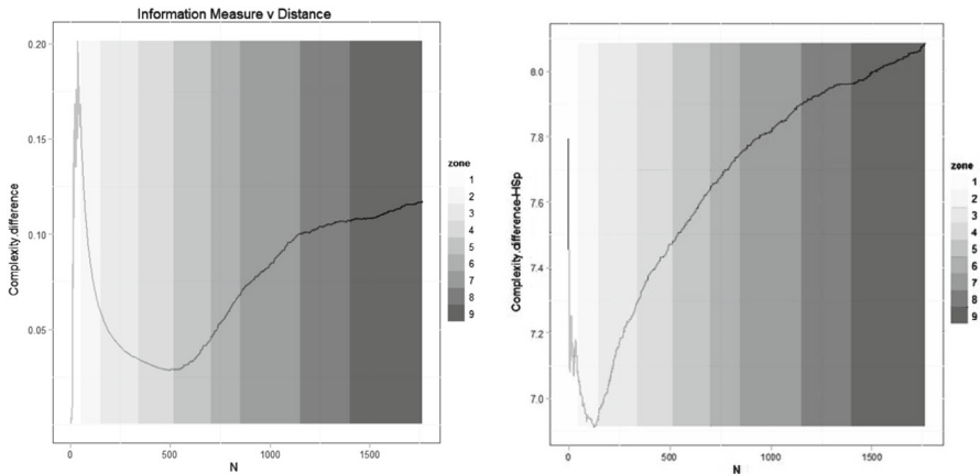
Fig. 11 The information difference H_{\max} - H and the information difference minus spatial entropy
