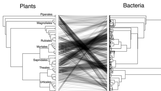
Fig. 4. Cophylogeny of host plants ( Left ) and phyllosphere bacteria ( Right ) on Barro Colorado Island, Panama. Lines connecting tips on the phylogenies indicate plant-bacterial associations that were stronger than expected according to a host-parasite coevolution test [ P < 0.05 (38)].
