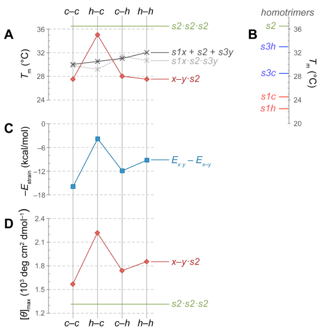
Figure 5. Comparison of experimental and computational data for x - y : s 2 and related triple helices. (A) Experimental (red and black) and calculated (gray) T_m values for heterotrimers. (B) Experimental T_m values for homotrimers. (C) Calculated strain energy, plotted as -E_{\text{strain}} to simplify comparisons with experimental data. (D) [\theta]_{\text{max}} from CD spectra acquired at 4 °C. Values for s 2 (green) are included in panels A, B, and D for comparison.
