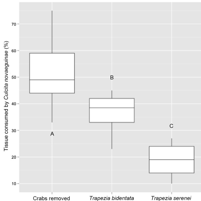
Figure 2 Percentage of coral tissue volume proxy consumed by Culcita novaeguinae in corals hosting the large size-class of Trapezia bidentata and Trapezia serenei . Letters indicate post-hoc statistically significant differences between groups.
