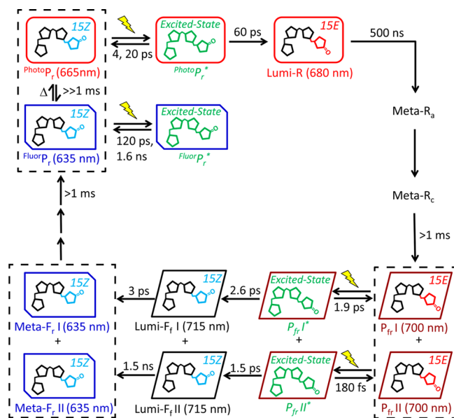
Figure 9. Scheme of the total Cph1 \Delta photocycle including both forward (P r to P fr ) and reverse (P fr to P r ). The spectrally and kinetically distinct fluorescent (FluorP r ) and photoactive (PhotoP r ) P r subpopulations are in slow equilibrium ( \gg 1 ms), which make up the overall P r state. The light-activated pathways are indicated by photoexcitation (yellow light sign) and subsequent evolution via thermally activated steps (solid arrows). The evolution of P fr to Lumi-F r to Lumi-F r occurs via heterogeneous pathways with different reaction kinetics and yields. Populations enclosed within black boxes indicate inhomogeneous coexisting populations.
