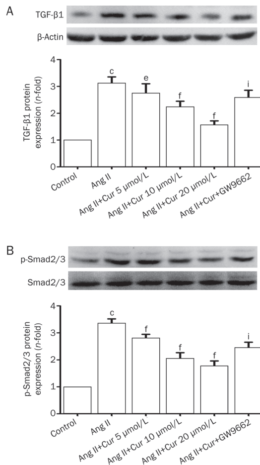
Figure 7. Cur inhibited Ang II-induced activation of TGF- \beta 1/Smad2/3 signaling pathway in CFs. The cells were pretreated with Cur (5, 10, and 20 \mu mol/L) and subsequently stimulated with Ang II (0.1 \mu mol/L) for another 24 h. A Western blotting assay was used to measure the expression of TGF- \beta 1 (A) and the phosphorylation of Smad2/3 (B). Data are presented as the mean \pm SEM of three independent experiments. c P <0.01 vs control. f P <0.01 vs Ang II. i P <0.01 vs Ang II+Cur 20 \mu mol/L.
