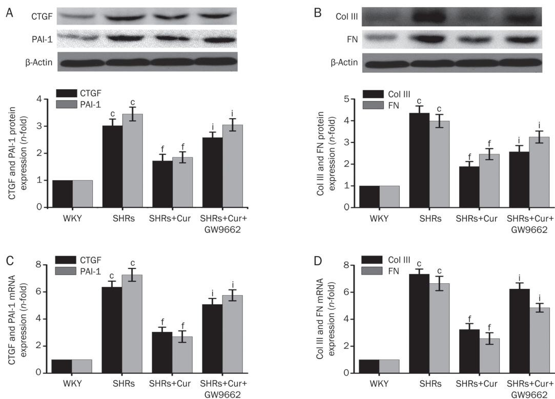
Figure 2. Cur downregulated mRNA and protein expression of CTGF, PAI-1, Col III, and FN in SHRs. WKY rats were used as controls, and SHRs were treated with saline, Cur (100 mg/kg 1 ·d 1 ), or Cur (100 mg/kg 1 ·d 1 )+GW9662 (10 mg/kg 1 ·d 1 ) by oral gavage for 12 weeks. Western blotting was used to measure the expression of CTGF (A), PAI-1 (A), FN (B), and Col III (B). The mRNA expression of CTGF (C), PAI-1 (C), FN (D), and Col III (D) was detected by real-time PCR ( n =8 rats, each group). Data are presented as the mean±SEM of three independent experiments. c P <0.01 vs WKY. f P <0.01 vs SHRs. i P <0.01 vs SHRs+Cur.
