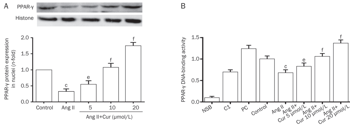
Figure 4. Cur increased the activation of PPAR- \gamma in Ang II-induced CFs. The cells were pretreated with Cur (5, 10, and 20 \mu\text{mol/L} ) for 1 h, and subsequently stimulated with Ang II (0.1 \mu\text{mol/L} ) for 24 h. Nuclear protein was extracted, and the expression of PPAR- \gamma was subsequently measured using Western blotting (A). PPAR- \gamma activation was detected by DNA-binding assay using a PPAR- \gamma transcription assay kit (B). NSB: nonspecific binding; C1: competitor; PC: positive control. Data are presented as the mean \pm SEM of three independent experiments. c P < 0.01 vs control. e P < 0.05 , f P < 0.01 vs Ang II. l P < 0.01 vs Ang II+Cur 20 \mu\text{mol/L} .
