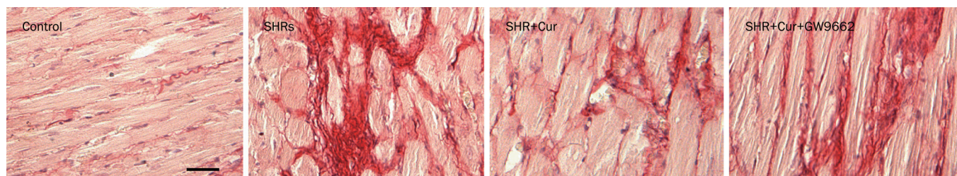
Figure 1. Cur decreased collagen deposition in the left ventricles of SHRs. WKY rats were used as controls, and SHRs were treated with saline, Cur ( 100 \text{ mg}\cdot\text{kg}^{-1}\cdot\text{d}^{-1} ), or Cur ( 100 \text{ mg}\cdot\text{kg}^{-1}\cdot\text{d}^{-1} )+GW9662 ( 10 \text{ mg}\cdot\text{kg}^{-1}\cdot\text{d}^{-1} ) by oral gavage for 12 weeks. Sirius Red staining was used to analyze the levels of collagen deposition in the left ventricles of WKY or SHRs ( n=8 rats, each group). Scale bar: 100 \mu\text{m} . WKY: Wistar Kyoto rats; SHRs: spontaneously hypertensive rats.
