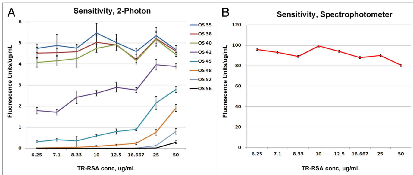
Figure 4. Effect of increasing offsets on sensitivity. Intensity data from Figure 2 was normalized to the individual concentrations to evaluate sensitivity. (A) The sensitivity values expressed as fluorescence units/ \mu\text{g/mL} remain relatively constant for offsets between 35–40, even at the lowest concentration of 6.25 \mu\text{g/mL} of TR-RSA. In contrast, the sensitivity of the remaining higher offsets starts low at the lowest concentration and climbs gradually. The two lowest offsets (52 and 56) show no appreciable detection capabilities until a concentration of \sim 16.67 \mu\text{g/mL} TR-RSA. The sensitivity values for the spectrophotometer shown in (B) denote a curve virtually identical to offsets 35–40 for the varying TR-RSA concentrations examined.
