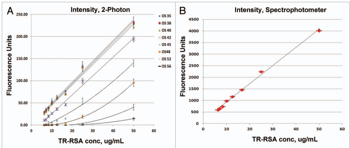
Figure 2. Effect of higher offsets on the linearity of detection. Fluorescence intensity graphs generated from the 2-photon microscopy in vitro images shows a loss of linearity for the concentrations of Texas Red rat serum albumin (TR-RSA) as the offsets increase. (A) The intensity profiles for offsets 35–42 appear to remain linear throughout the range of concentrations of TR-RSA used. For the remaining offsets, 45 through 56, the intensity curves conform to a polynomial function with less sensitivity noted. (B) The intensity profile generated for the solutions of TR-RSA using the Spectramax M5 spectrophotometer are shown. Here, a linear relationship between the different concentrations of TR-RSA was observed.
