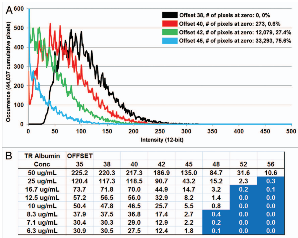
Figure 3. Effect of higher offsets on pixel values. Histograms generated from the 12.5 ug/mL TR-RSA concentration images show an increasing number of individual pixels with values of zero as offset is increased. (A) Histograms for offsets 38, 40, 42 and 45 are shown in black, red, green and blue, respectively. The Y-axis showing the number of occurrences for a specific pixel value is truncated at 600. The total number of pixels counted in the area was 44,037. Images taken at offsets 42 and 45 had 12,079 and 33,293 pixels with a value of zero, respectively. Note the bell shaped curves seen for offsets 38 and 40, which become sharply rising curves peaking with increasing values at zero for offsets 42 and 45. (B) A table shows average intensity values for each offset at the varying concentrations of TR-RSA. Average intensity values fall below zero at higher offsets (shown in blue) and at lower concentrations where fluorescence becomes weaker. Note the proportional drop in fluorescence between concentrations of TR-RSA at the lower offsets while higher offsets show a disproportionately larger decrease in intensity values as the concentration of TR-RSA decreases.
