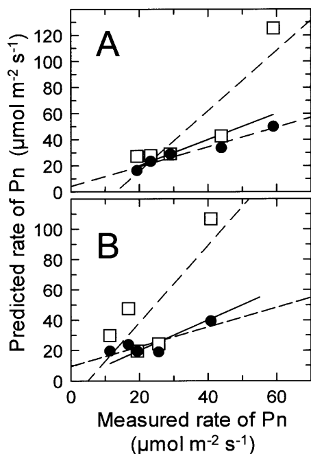
Figure 2. Relationship between the measured and predicted rates of Pn in nonstressed and heat stressed leaves of creosote bush and Antarctic hairgrass at ambient and elevated C_i . The predicted rates of Pn for creosote bush (A) and Antarctic hairgrass (B) were calculated from the kinetic properties of Rubisco with (●) and without (□) adjustment for the measured changes in Rubisco activation. The two dashed lines show the linear regression of the relationship between measured and predicted rates of Pn with (●) and without (□) adjustment for changes in Rubisco activation. Values for Pn and Rubisco activation, as well as the conditions of temperature, C_i , and O_2 , are from Tables I (A) and II (B). The solid line denotes a 1:1 relationship between measured and predicted rates.
