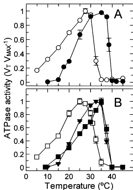
Figure 6. Effect of temperature on the activity of recombinant activase from plants native to warm and cold regions. A, The ATPase activity of recombinant Antarctic hairgrass (○) and creosote bush (●) activase was measured at the indicated temperatures. B, The ATPase activity of recombinant spinach (□), tobacco (■), and cotton (▼) activase was measured at the indicated temperatures. Results are expressed as V_T V_{MAX}^{-1} , the ratio of the activities at the indicated temperature ( V_T ) to the activity at the temperature optimum ( V_{MAX} ). Maximum rates of ATP hydrolysis were 0.9, 0.56, 0.75, 0.86, and 0.59 units mg\ protein^{-1} for activase from Antarctic hairgrass, creosote bush, spinach, tobacco, and cotton, respectively.
