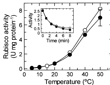
Figure 5. Effect of temperature on the carboxylase activity of Rubisco isolated from Antarctic hairgrass and creosote bush. The carboxylase activity of Rubisco from Antarctic hairgrass ( \circ ) and creosote bush ( \bullet ) was determined at the indicated temperatures. The enzyme was incubated with 30 mM NaHCO 3 and 10 mM MgCl 2 to fully carbamylated the enzyme prior to assay. Inset, Time course of inactivation of Rubisco under catalytic conditions. Fully carbamylated Rubisco from Antarctic hairgrass ( \circ ) and creosote bush ( \bullet ) was incubated at 40°C in the presence of RuBP, and residual activity was determined at 30°C at the indicated times.
