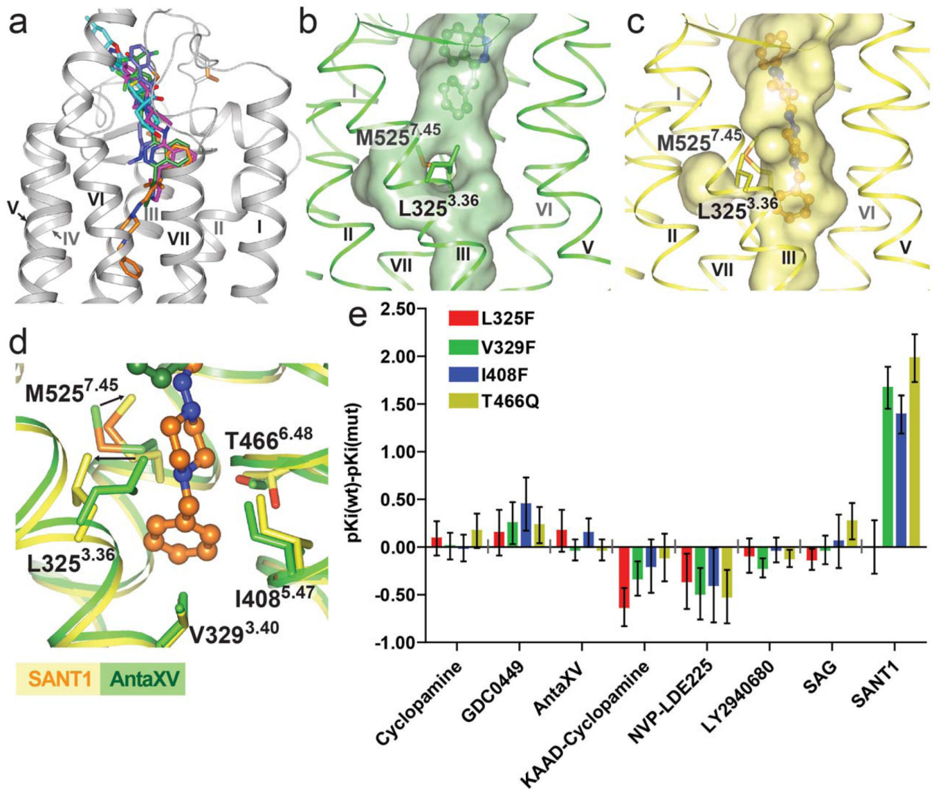
Figure 2. The deep binding pocket of SANTI1
