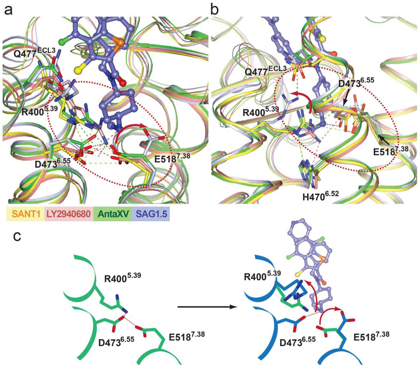
Figure 4. Agonist SAG1.5 induced conformational changes in the ligand binding pocket (a) Superposition of the ligand binding pocket residues of different structures of SMO. The receptor structure and side chain carbons are shown for SMO_Anta XV (green), SMO_SANT1 (yellow), SMO_LY2940680 (salmon; PDB id: 4JKV, molecule A), and SMO_SAG1.5 (light blue) structures. The ligand SAG1.5 is shown as light blue carbons. The hydrogen bond interactions between side chains are shown as dashed lines in the corresponding color of each structure. (b) A different view of the superposition of the ligand binding pocket residues. H470 6.52 which interacts with R400 5.39 in antagonist bound structures is shown. Red arrows (in (a) and (b)) are shown to indicate the conformational changes of E518 7.38 and R400 5.39 induced by SAG1.5 binding. (c) Schematic presentation of agonist induced conformation change: green is antagonist bound state, while blue is agonist bound state.
