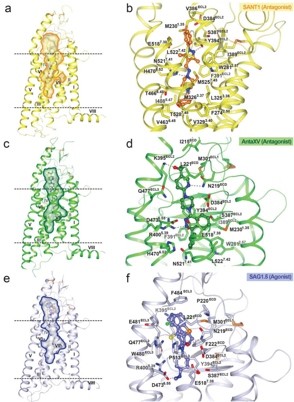
Figure 1. Overall structures of SMO receptor bound to different ligands and the ligand binding pockets
