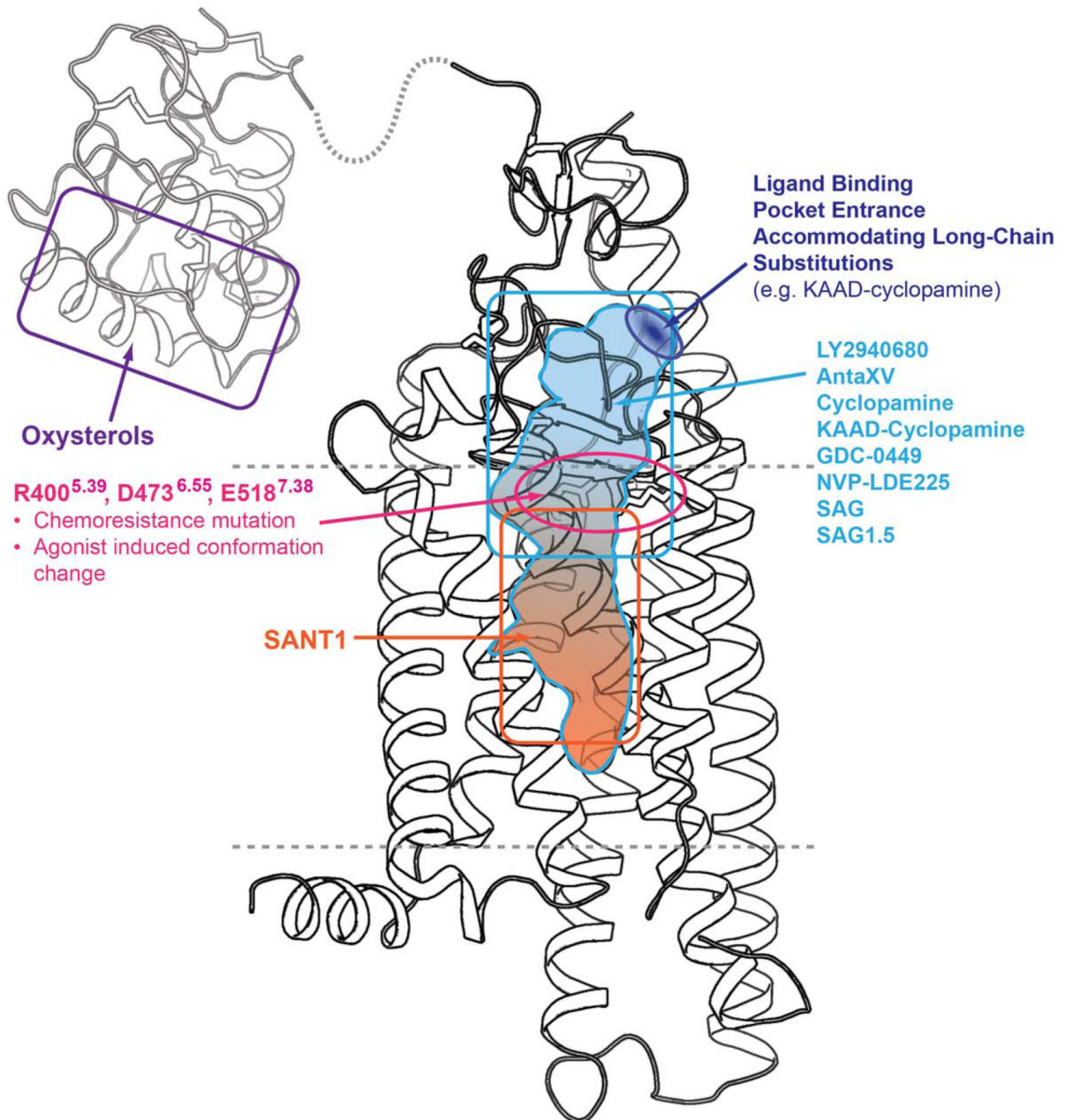
Figure 5. Map of the structural basis for the modulation of SMO by small molecules The N terminal CRD domain is shown using the CRD of zebrafish SMO (PDB id: 4C79). The boundaries of the membrane bilayer are shown as dashed lines.
