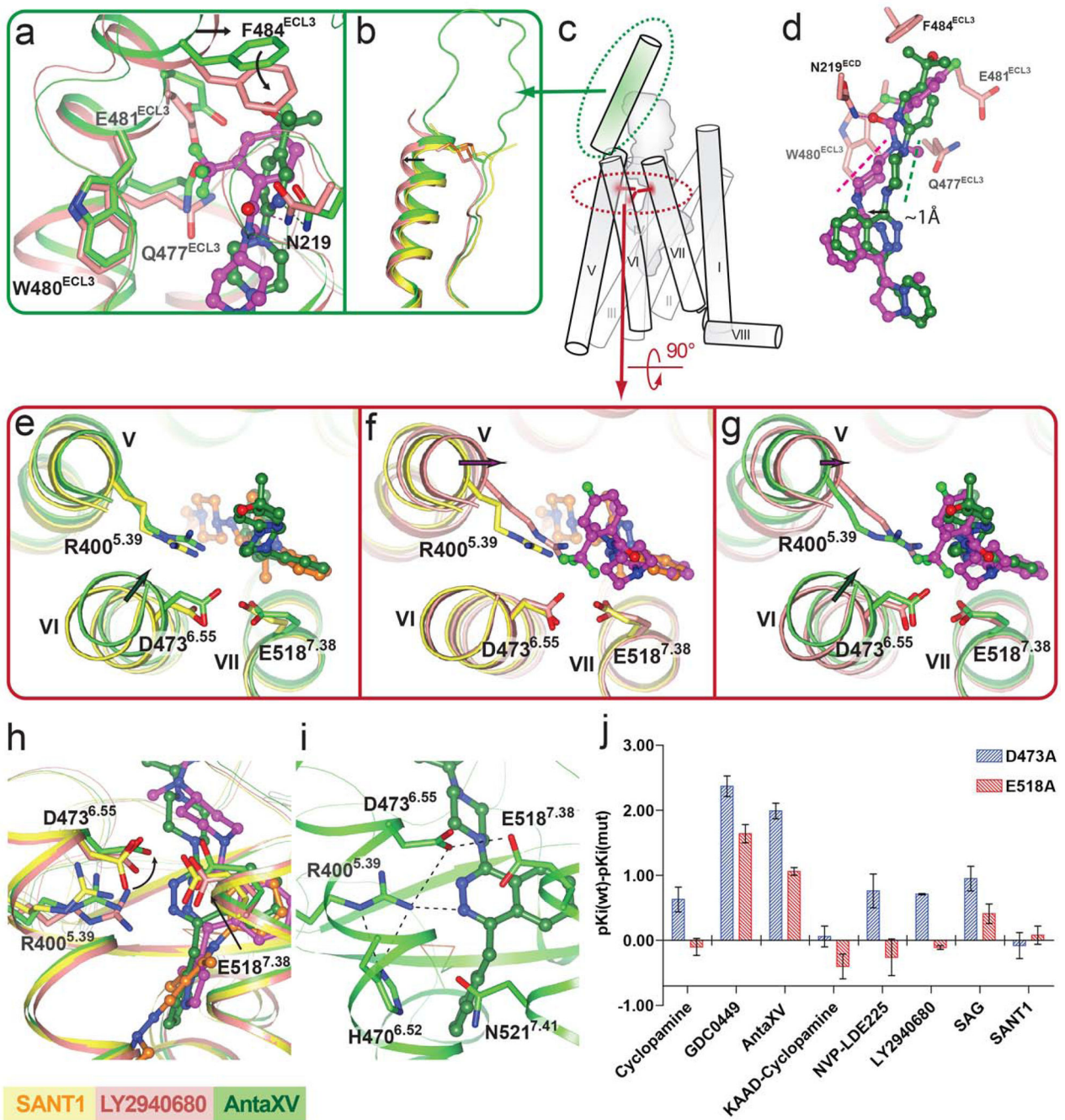
Figure 3. D473 6.55 plays different roles in the recognition of Anta XV and LY2940680 (a)–(i) The receptor structures in SMO_Anta XV, SMO_SANT1 and SMO_LY2940680 (PDB id: 4JKV, molecule A) complexes are shown in green, yellow and salmon, respectively. Ligand structures of Anta XV, SANT1 and LY2940680 are shown in green, orange and magenta carbons, respectively. (a) Superposition of SMO_LY2940680 and SMO_Anta XV structures near ECL3. The conformational change of F484 ECL3 induced by LY2940680 binding is shown by an arrow. See also Supplementary Figure 4 for comparison with SMO_SANT1 structure. (b) Superposition of the SMO_SANT1, SMO_Anta XV and
