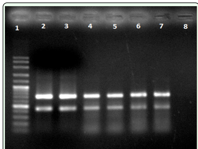
Figure 1. Amplifications of COI and Cyt b genes produced 710 bp and 440 bp of multiplex PCR products from braconid species. Lane 1: 100 bp DNA ladder; Lanes 2 and 3: Diachasmimorpha longicaudata (annealing temperature, T_a = 47^\circ \text{C} ); Lanes 4 and 5: Fopius arisanus ( T_a = 50^\circ \text{C} ); Lane 6: Psytalia incisi ( T_a = 50^\circ \text{C} ); Lane 7: Fopius sp. ( T_a = 50^\circ \text{C} ); Lane 8: negative control. High quality figures are available online.
