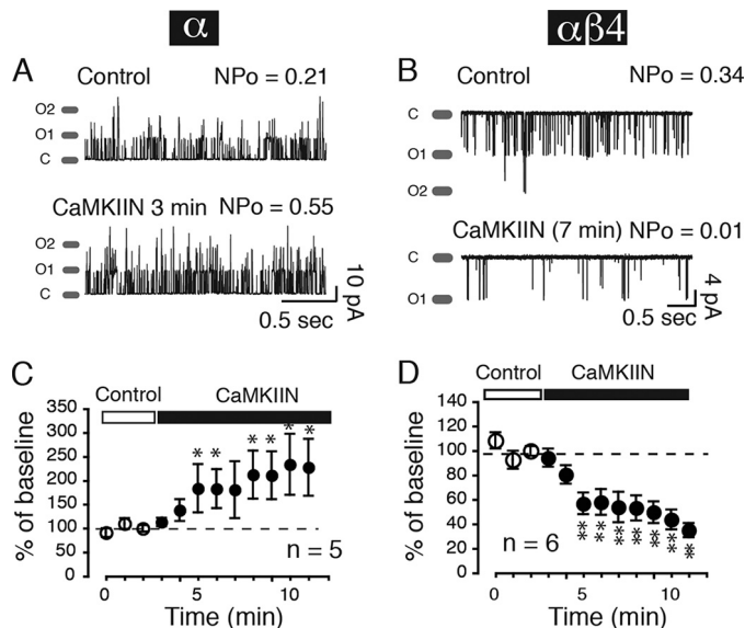
FIGURE 5. Effects of inhibiting CaMKII on \alpha and \alpha\beta 4 BK channel open probability. A and B, sample traces of BK channel activity before and during drug exposure. The right-hand side of each trace shows the NP_o measured during 20 s recording. C and D, average BK channel activity before (control) and during drug exposure (filled bars). The dashed line shows the baseline control level. Number of patches tested in each condition is indicated by the n value shown in the lower left part of the graphs. Asterisks represent statistically significant differences from baseline: * indicates p \leq 0.05 , and ** indicates p \leq 0.01 .
