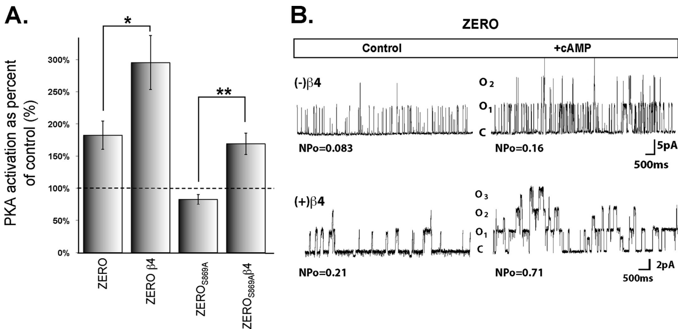
FIGURE 4. Effect of PKA activation on \alpha and \alpha\beta 4 BK channel NP_o in the wild-type channel and in channel expressing S869A mutation in HEK 293 recorded using excised patches. A, bar graph quantifying NP_o of individual inside-out patch clamp recordings with 0.1 mM cAMP in the bath solution containing 1 mM ATP. The graph is plotted showing PKA activation as percent of control (untreated). The dashed line shows the baseline control level. B, representative traces of \alpha ( hp = +40 mV) and \alpha\beta 4 ( hp = +20 mV) BK channel activity before (control) and during 0.1 mM cAMP exposure (6 min). The numbers below the traces indicate open probability. Number of patches tested, one patch per cell, in each condition was n = 4 . Asterisks represent statistically significant differences: *, p \leq 0.05 , and **, p \leq 0.01 .
