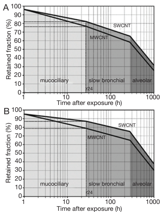
Figure 5 Course of clearance with its single clearance phases computed for average SWCNT ( d_{ae} = 10 nm) and average MWCNT ( d_{ae} = 100 nm): (A) clearance following particle deposition after sitting breathing; (B) clearance following particle deposition after light-work breathing. SWCNT, single-walled carbon nanotubes; MWCNT, multi-walled carbon nanotubes.
