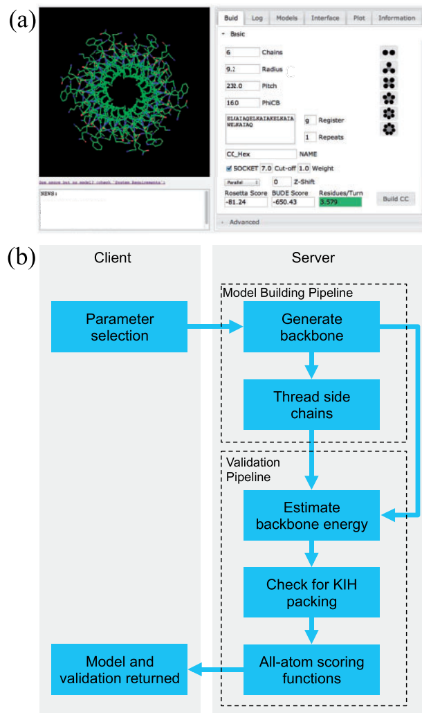
Fig. 2. Overall architecture, appearance and workflow of CCBuilder. (a) GUI displaying the molecule viewer and the ‘Basic’ build tab, which contains fields for parameter entry and displays the returned model scoring. (b) Application architecture and workflow
