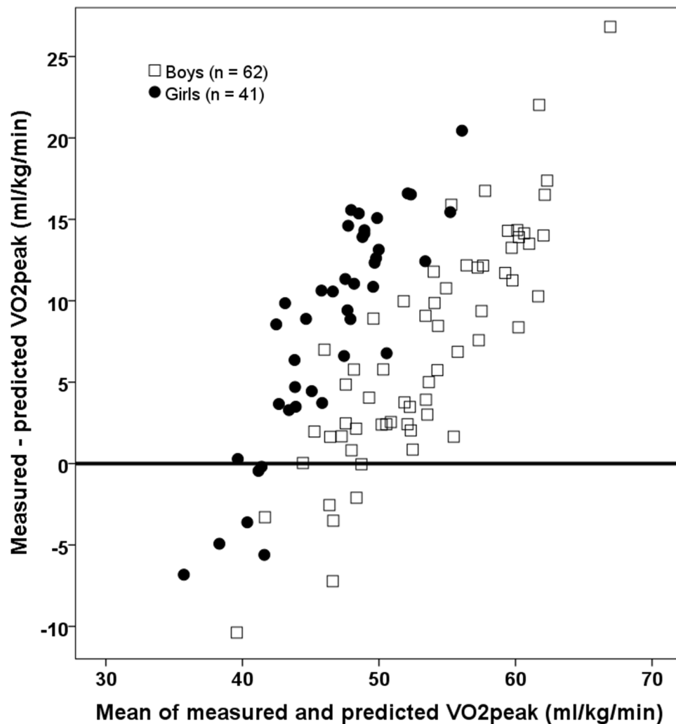
Figure 2. Bland Altman plots showing differences between measured VO_{2peak} and predicted VO_{2peak} from Andersen et al. ( VO_{2peak} = 18.38 + 0.033 * \text{Andersen test} - 5.92 * \text{gender} ) as a function of the mean of the two values.
