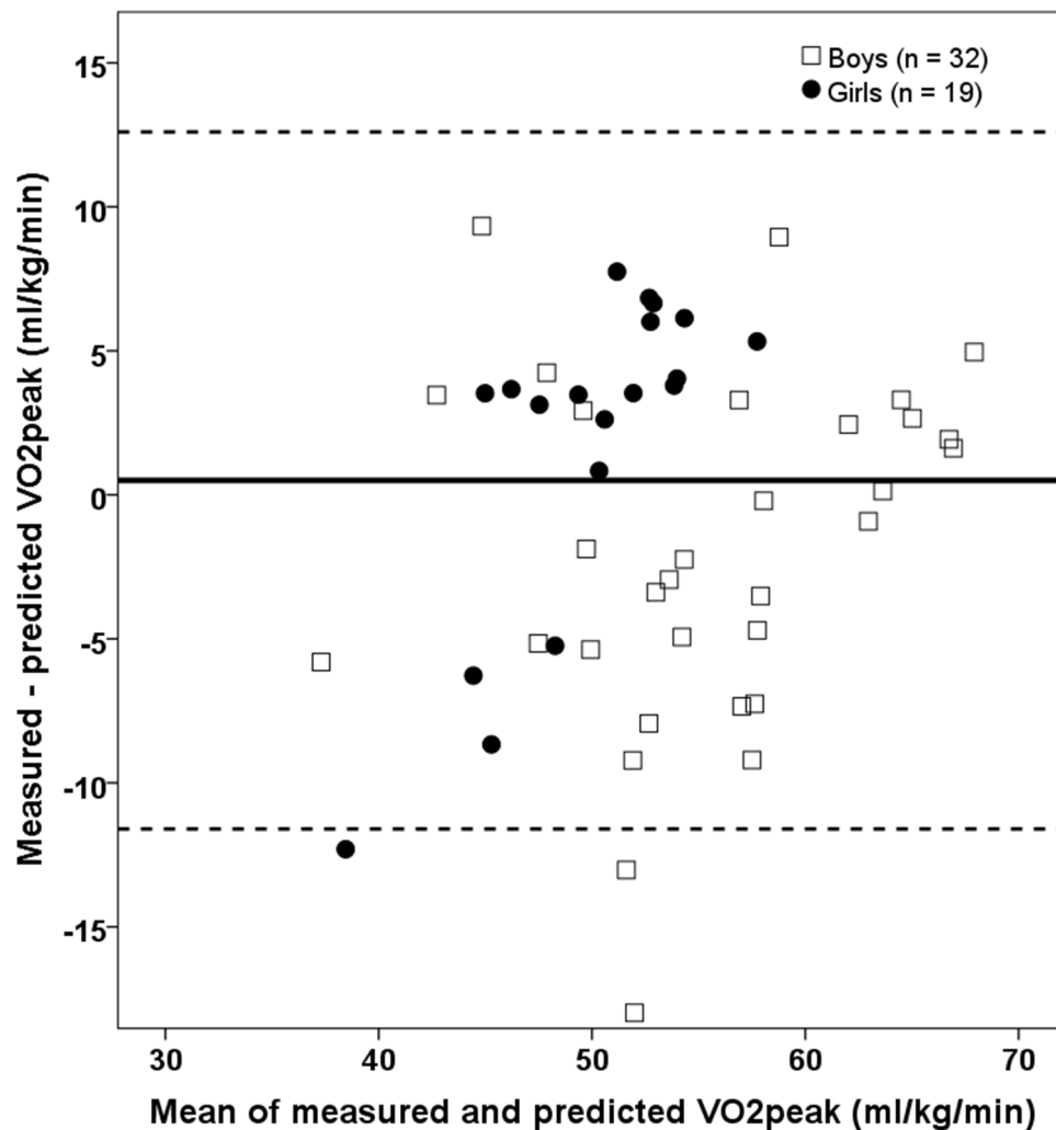
Figure 3. Bland Altman plots showing differences between measured VO_{2peak} and predicted VO_{2peak} as a function of the mean of the two values in class 2 (testing dataset) based on the regression equation derived from class 1 (training dataset) ( VO_{2peak} = 22.887 + 0.052 * \text{Andersen test} - 5.632 * \text{gender} - 0.386 * \text{body weight} ). The solid line is the mean difference; dotted line is limits of agreement ( \text{bias} \pm 1.96 * \text{SD} of the difference). doi:10.1371/journal.pone.0110492.g003
