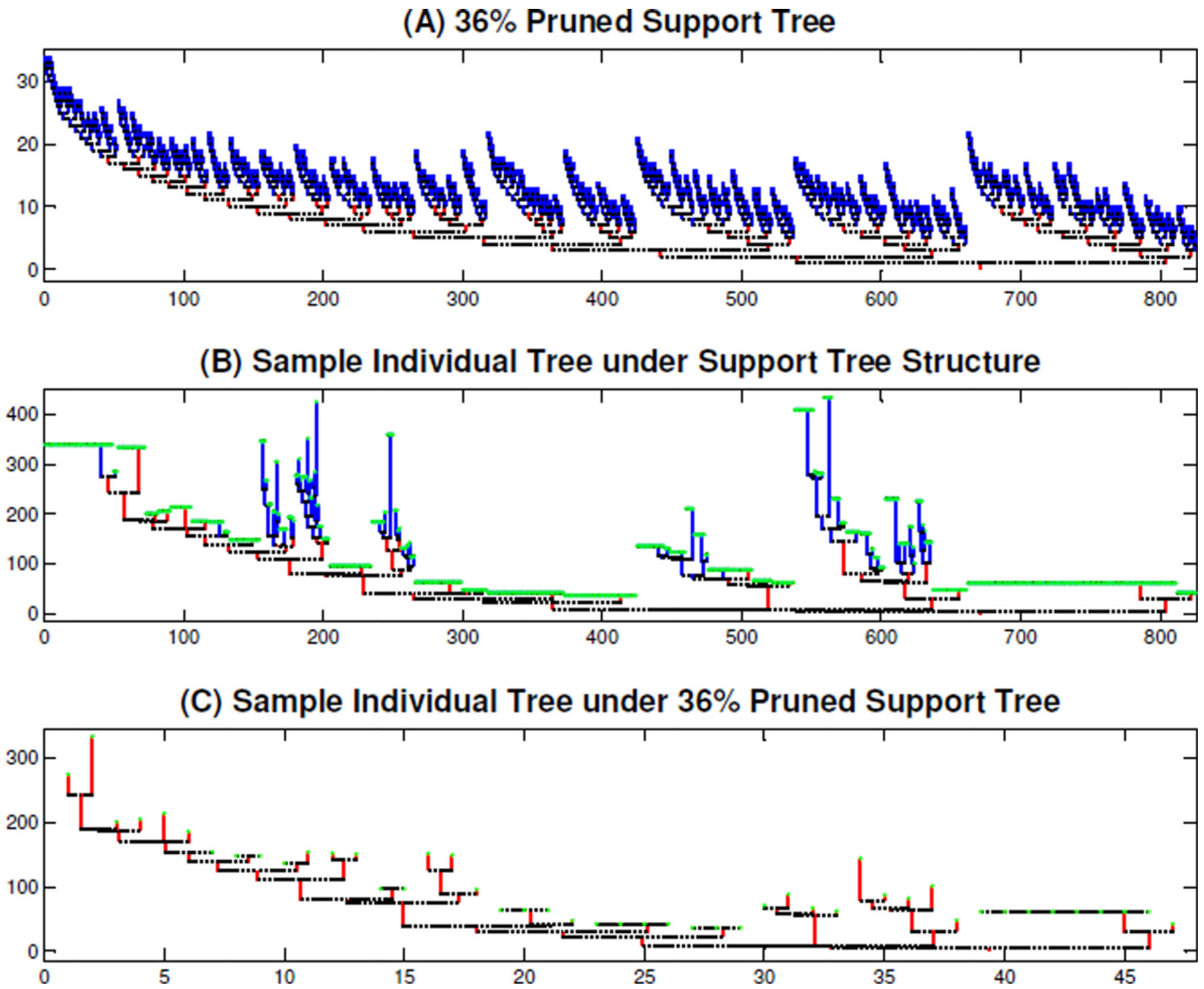
Figure 13. Illustration of Tree Pruning, for Support Tree and an Individual. The red tree in Panel (A) is the 36% pruned support tree whose branches appear in at least 36 percent of the individual trees. Panel (B) is an individual tree under the support tree structure, where the missing branches are colored green, the non-missing branches that appear in the 36% pruned support tree are red, and the non-missing branches that are not in the pruned support tree are blue. Panel (C) is the corresponding individual 36% pruned tree that contains the red branches and the missing branches that appear in the 36% pruned support tree in the top panel.
