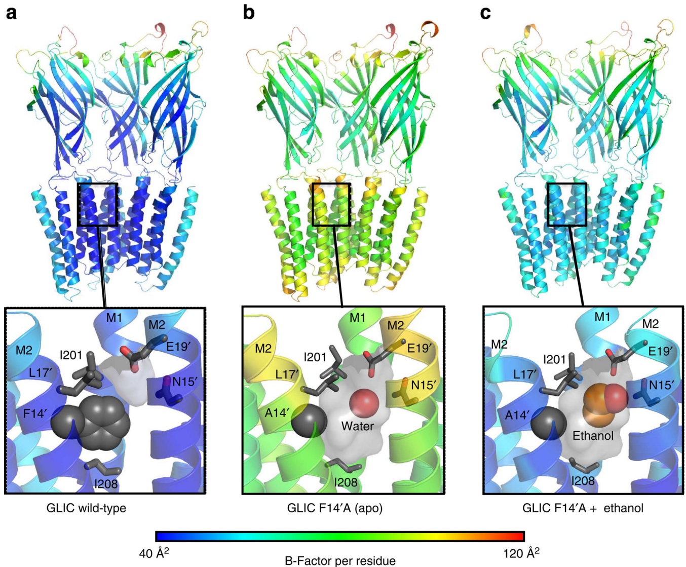
Figure 1. X-ray structures of wild-type and ethanol-sensitized GLIC
