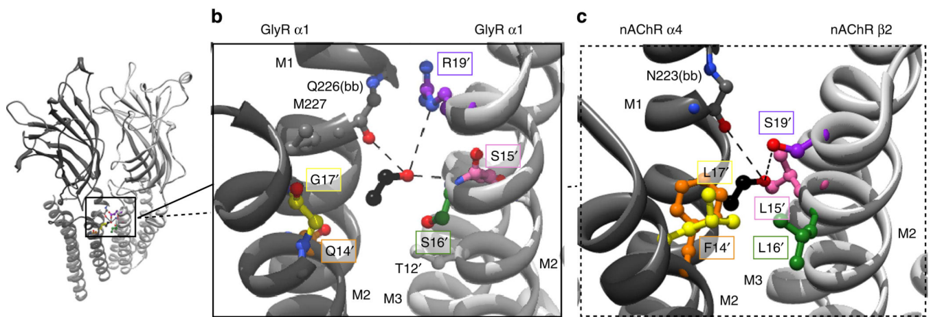
Figure 5. Alignment of GLIC F14'A with human alcohol targets
