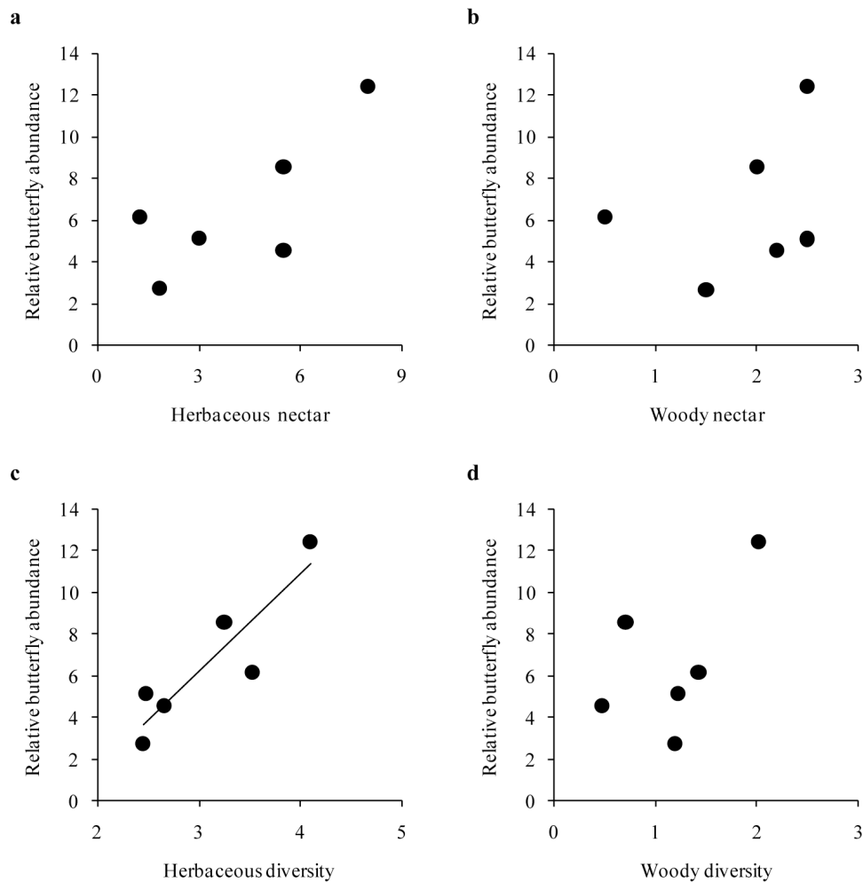
Figure 3. Relationship between potential herbaceous (a) or woody (b) nectar availability and herbaceous (c) or woody (d) plant diversity with relative butterfly abundance within sclerophyllous sites. N = 6 . Regressions lines are shown when significant (see results section). High quality figures are available online.
