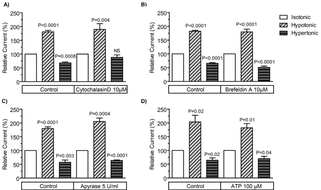
Figure 4. Mechanisms for cell volume regulation of Slick K + channels. Slick channels were co-expressed with AQP1 in Xenopus laevis oocytes and the channels were activated by depolarizations to +80 mV for 500 ms (holding potential: -80 mV). In all cases, the maximal currents (at the end of the depolarization period) were measured in isotonic, hypotonic and hypertonic media and are shown as relative changes in the current during cell swelling (hatched bars) and shrinkage (horizontal bars) as compared to the current under isotonic conditions (open bar). The figures show the effect of (A) cytochalasin D (10 μM, preincubation 24 hours), (B) Brefeldin A (10 μM, preincubation 8 hours), (C) Apyrase (5 U/ml) and (D) ATP (100 μM). All values are given as means ± SEM (n = 6–8). doi:10.1371/journal.pone.0110833.g004
