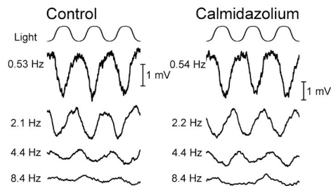
Figure 9. Synaptic responses to sinusoidal stimuli are reduced by inhibition of CaM. (A) In control voltage-clamp recordings of an HC (left), response amplitude to a sinusoidal light stimulus decreased with increasing stimulus frequency. In recordings from a different HC (right), response amplitude in the presence of 20 \mu M calmidazolium declined at lower frequencies relative to control recordings. (B) HC group data normalized to the response amplitude at 0.5 Hz. In the presence of calmidazolium, responses fell off at lower frequencies than in controls. (C) A similar effect was seen in recordings from On BCs. (D) Perforated patch current-clamp recordings of responses from two separate cones to sinusoidal light stimuli in control conditions (left) and in the presence of the CaM inhibitor calmidazolium (20 \mu M; right). (E) Under control conditions, the cone light responses were exclusively low pass, peaking at the lowest frequency tested (0.5 Hz) and falling off at higher frequencies. In the presence of calmidazolium, the responses were no different than in control conditions. (F) In paired recordings of cones and HCs, cones were stimulated with a 0.5–16-Hz sinusoidal voltage-clamp command (20 mV peak-to-peak around a holding potential of -40 mV). Data were normalized to responses at 1 Hz. When cones were dialyzed with the MLCK-control peptide (20 \mu M; n = 8 ), HC responses were band-pass, peaking at 3–4 Hz and falling off at higher or lower frequencies. When cones were dialyzed with the MLCK peptide (gray; 20 \mu M), response amplitude fell off at lower frequencies than in controls. Mean \pm SEM is shown. *, P < 0.05 ; **, P < 0.01 .
