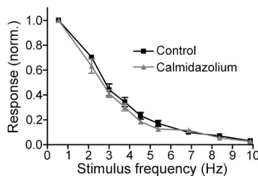
Figure 9. Synaptic responses to sinusoidal stimuli are reduced by inhibition of CaM. (A) In control voltage-clamp recordings of an HC (left), response amplitude to a sinusoidal light stimulus decreased with increasing stimulus frequency. In recordings from a different HC (right), response amplitude in the presence of 20 \mu M calmidazolium declined at lower frequencies relative to control recordings. (B) HC group data normalized to the response amplitude at 0.5 Hz. In the presence of calmidazolium, responses fell off at lower frequencies than in controls. (C) A similar effect was seen in recordings from On BCs. (D) Perforated patch current-clamp recordings of responses from two separate cones to sinusoidal light stimuli in control conditions (left) and in the presence of the CaM inhibitor calmidazolium (20 \mu M; right). (E) Under control conditions, the cone light responses were exclusively low pass, peaking at the lowest frequency tested (0.5 Hz) and falling off at higher frequencies. In the presence of calmidazolium, the responses were no different than in control conditions. (F) In paired recordings of cones and HCs, cones were stimulated with a 0.5–16-Hz sinusoidal voltage-clamp command (20 mV peak-to-peak around a holding potential of -40 mV). Data were normalized to responses at 1 Hz. When cones were dialyzed with the MLCK-control peptide (20 \mu M; n = 8 ), HC responses were band-pass, peaking at 3–4 Hz and falling off at higher or lower frequencies. When cones were dialyzed with the MLCK peptide (gray; 20 \mu M), response amplitude fell off at lower frequencies than in controls. Mean \pm SEM is shown. *, P < 0.05 ; **, P < 0.01 .
