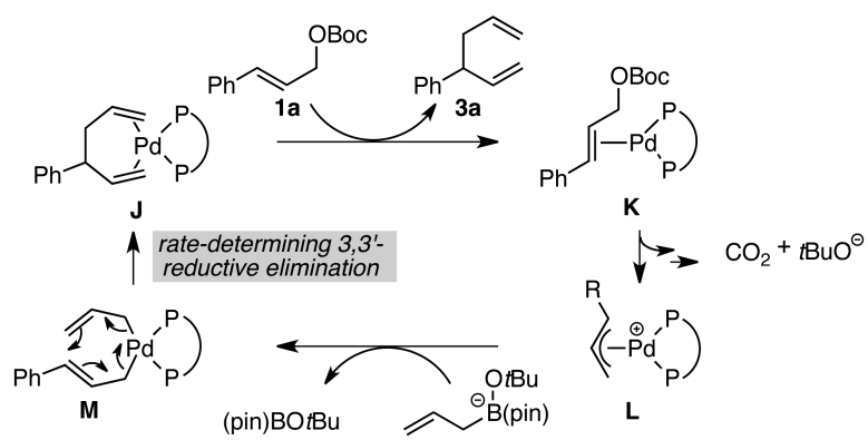
Scheme 2. Proposed Catalytic Cycle
