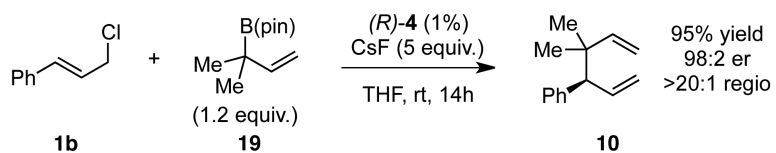
Scheme 6. Increased Reactivity with \alpha,\alpha -Disubstituted Allylboron Nucleophiles
