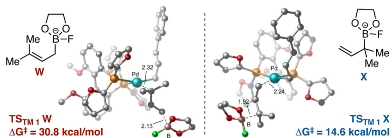
Figure 5. Calculated activation free energy for transmetalation of fluoride-activated 9 ( W , left) and 19 ( X , right) to GS 1 . B3LYP-PCM(THF)/LANL2DZ-6-31G** (298.15K).
