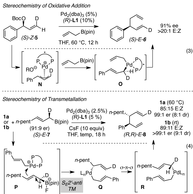
Scheme 3. Labeling Studies of Reaction Stereochemistry
