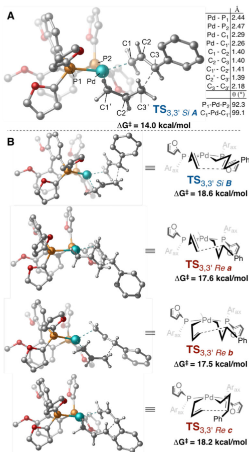
Figure 4. (A) Optimized structure and coordinates for TS 3,3' Si A (B) Activation energies relative to GS 2 for other possible allyl conformations during 3,3'-reductive elimination. B3LYP-PCM(THF)/LANL2DZ-6-31G** (333.15 K).
