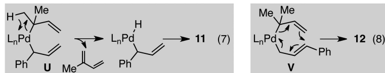
Scheme 5. Initial Results for Congested Bond Formations
