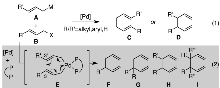
Scheme 1. Pd-Catalyzed Allyl-Allyl Couplings
