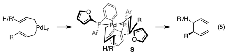
Scheme 4. Stereochemical Model for 3,3'-Reductive Elimination
