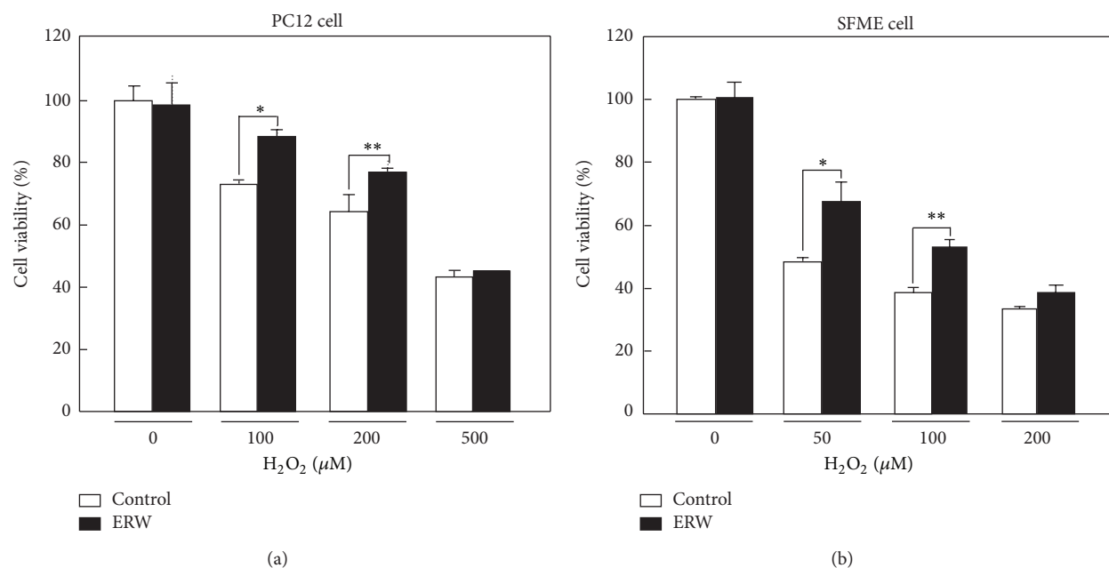
FIGURE 1: Suppressive effect of ERW against H 2 O 2 -induced cytotoxicity on PC12 and SFME cells. Viable cell numbers were measured using a WST-8 kit. (a) Pheochromocytoma PC12 cells were cultured in FBS/HS/DMEM medium with or without ERW and the number of surviving cells were set as controls. H 2 O 2 (100, 200 and 500 μM) was added to the control medium and it was cultured for 24 h. Viable cells were measured at 450 nm using a microtiter plate reader. (b) Serum-free mouse embryo (SFME) cells were cultured in a 1:1 mixture of DMEM: Ham's F12 medium with or without ERW and the number of surviving cells were set as controls. To the control medium, H 2 O 2 (50, 100 and 200 μM) was added and it was cultured for 24 h. Viable cells were measured at 450 nm using a microtiter plate reader. Data are presented as mean ± standard deviation (SD) for three independent experiments ( n = 3 each set). * P < 0.05 and ** P < 0.01 .
