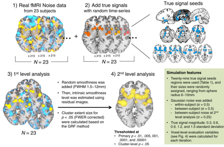
Fig. 3. The Simulation 2 procedure (Simulation 2 section). We conducted 100 iterations of second level analysis for each of 100 iterations of first level analysis (total 10,000 iterations). Real noise data are from Wager et al. (2009); see Simulation 2 section for details. FWER = family-wise error rate; FWHM = full width at half maximum; GRF = Gaussian random field.
