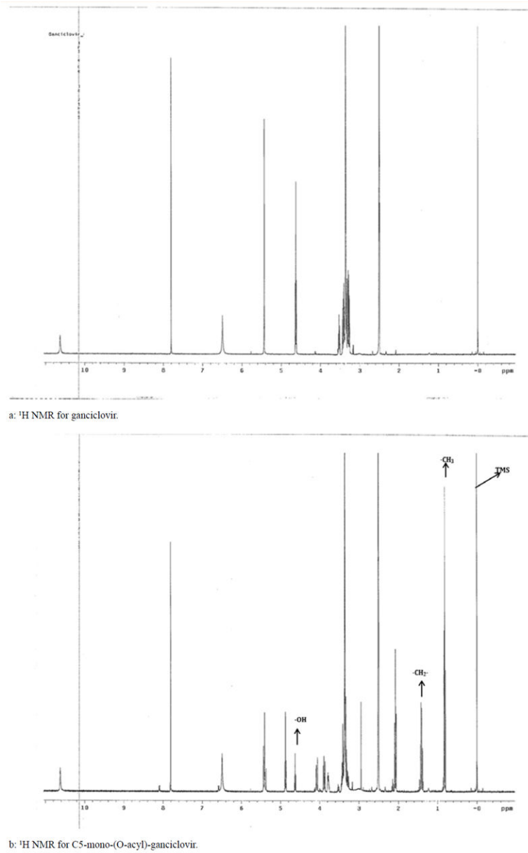
Figure 2. Proton ( ^1\text{H} ) NMR for ganciclovir and its mono lipid conjugate.
