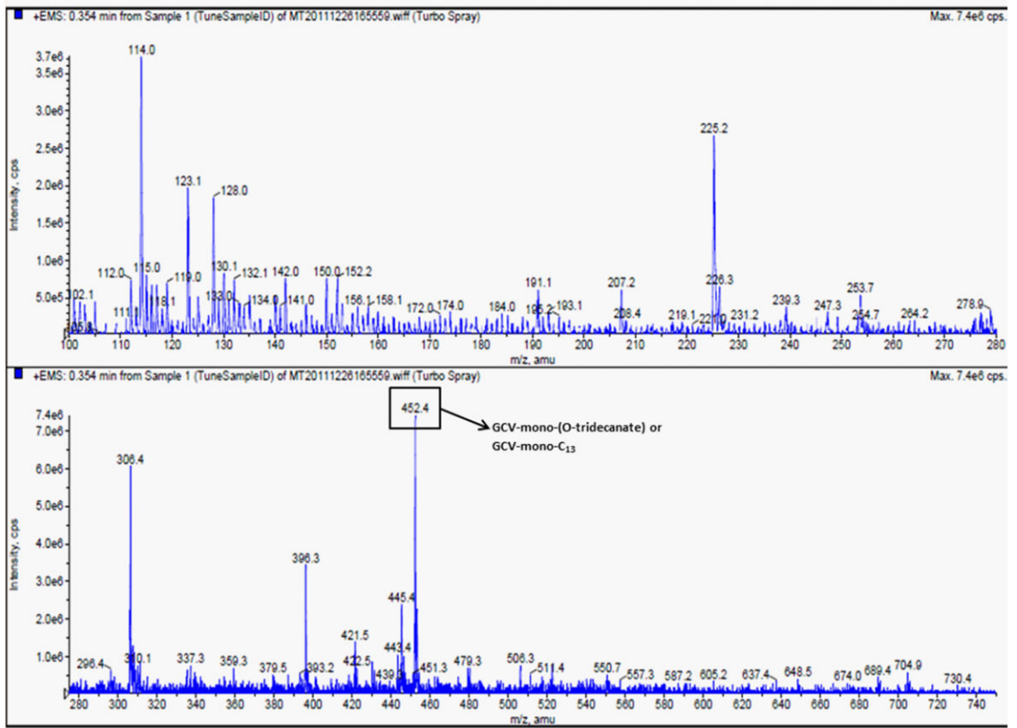
Figure 1. Mass spectral analysis for the purified prodrug ganciclovir-mono-(O-acyl)-C 13 .
