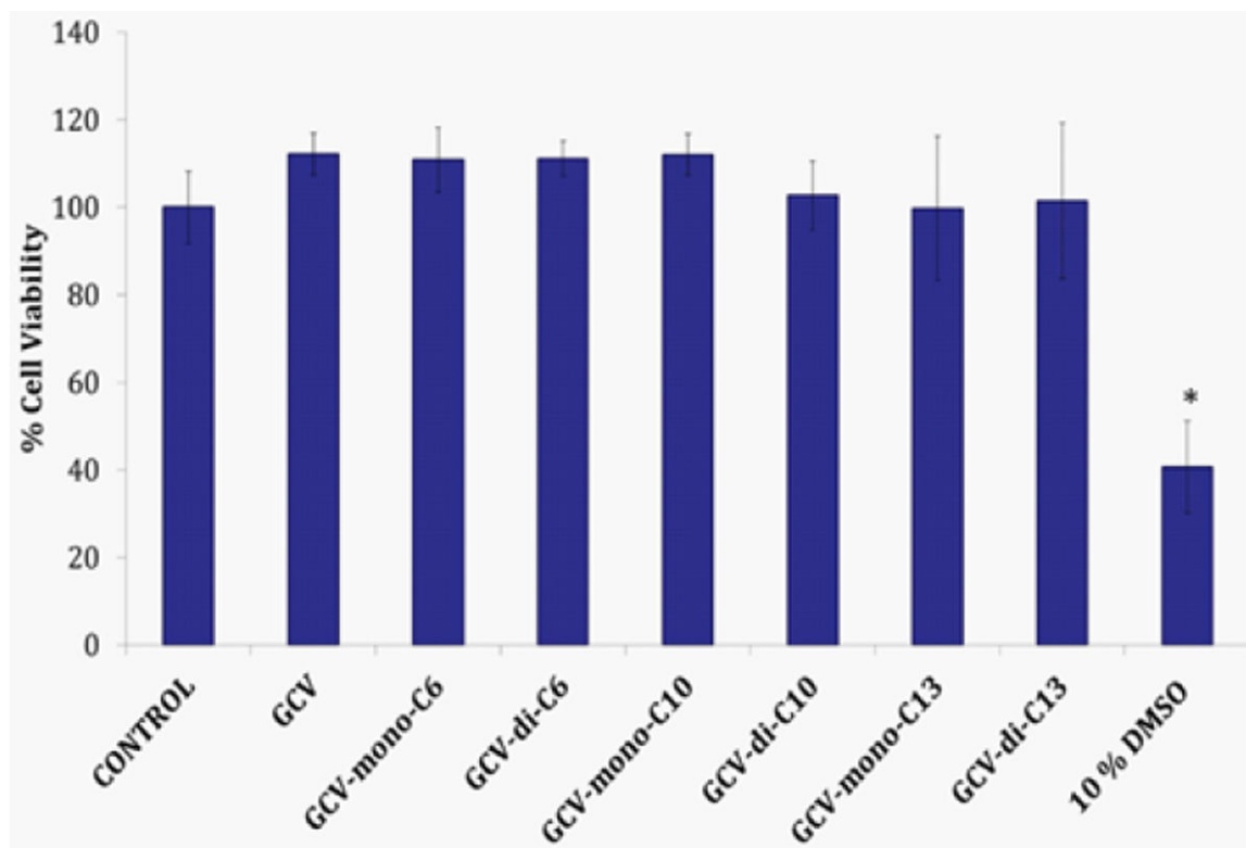
Figure 3. Ganciclovir (GCV) lipid prodrug cell proliferation studies on ARPE-19 cells. Cytotoxicity studies were conducted on ARPE-19 cells (N=8). Cells were treated with 100 \mu M of drug/prodrug solutions for 24 h. DMSO (10%) served as positive control and culture medium as negative control. Statistical analysis of p -value <0.05 is considered significant and represented with symbol “*”.
