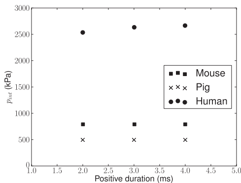
Fig. 6. Intracranial overpressure vs. time duration of the positive phase of the blast wave for peak incident overpressure p_{inc} = 200 kPa across mammalian species.
