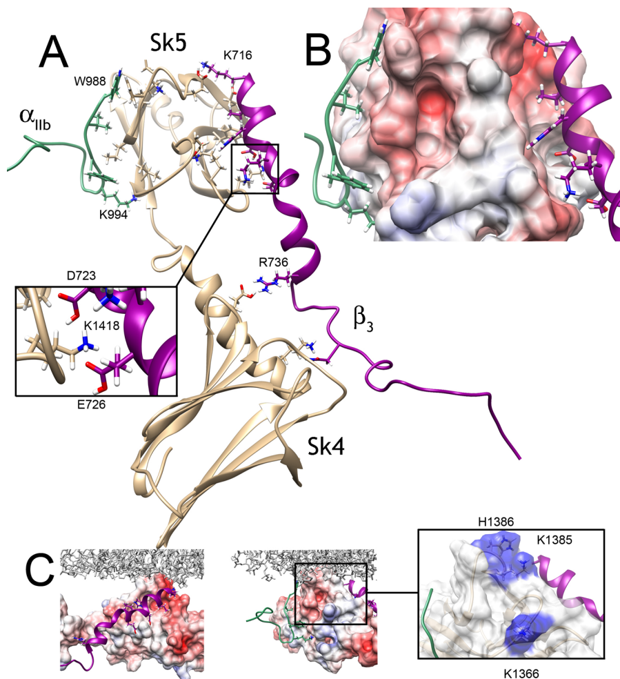
Figure 5. (A) Model of tertiary integrin/skelemin complex: Sk45 (tan) is shown bound to cytoplasmic tails of \alpha_{\text{IIB}} (green) and \beta_3 (purple) in ribbon presentation. Key residues are labeled. The inset shows a slightly rotated display of the hydrogen bonding network for a better view. (B) Zoomed view of the binding interface with Sk5 domain. The surface of Sk5 is colored based on its electrostatic potential. (C) The tertiary complex is arbitrarily placed with respect to the lipid bilayer represented by POPC and POPE mixture 27 shown in gray. Each side is shown to better visualize the binding pockets and potential orientation with the lipid bilayer. The inset depicts potentially positively charged residues of Sk5 domain (colored in blue) that may interact with the lipid bilayer.
