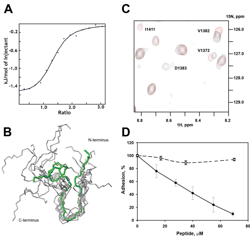
Figure 4. (A) ITC data for the Sk45 interaction with \alpha_{11b} fitted with a single binding site model. (B) The NMR ensemble of \alpha_{11b} cytoplasmic tail in the bound conformation as determined from trNOE data. The conformer used for docking is shown in green. (C) A region of the ^1\text{H} - ^{15}\text{N} HSQC spectra of Sk45 in absence (black) and presence of \beta_3 (red) at the protein/peptide ratio 1:3. Affected residues are labeled. (D) Effect of skelemin-derived peptide on \alpha_{11b}\beta_3 -expressing CHO cell adhesion. Microtiter wells were coated with 2.5 \mu\text{g}/\text{mL} of fibrinogen and postcoated with 1% BSA. Calcein-labeled \alpha_{11b}\beta_3 -expressing CHO cells were incubated with different concentration of THIVWYKDEREISVDEKHD ( \bullet ) or control EREISAAAKHD ( \circ ) peptides for 20 min at 22 ^\circ\text{C} . After 30 min at 37 ^\circ\text{C} , nonadherent cells were removed, and adhesion was determined. Data points are expressed as a percentage of control adhesion (in the absence of peptides) and are the mean of three individual experiments performed with triplicate determinations in each experiment.
