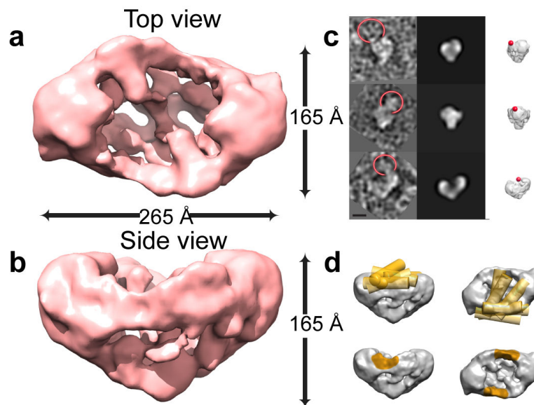
Figure 2. 3D reconstruction of BRCA2-RAD51 complex
