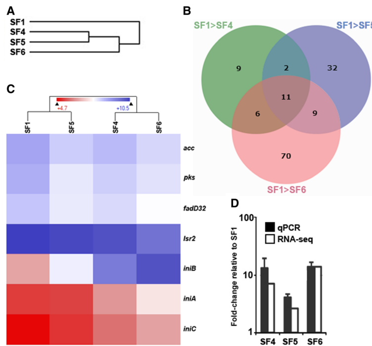
Figure 5 Differential gene expression in serial isolates. (A) Hierarchical clustering of total gene expression. (B) Venn diagram of differentially expressed genes in SF4, SF5 and SF6 relative to SF1. (C) Hierarchical clustering of interesting genes and operons (high and low expression indicated by blue and red coloring, respectively). (D) Fold change of iniB expression relative to SF1. qPCR, quantitative PCR.
