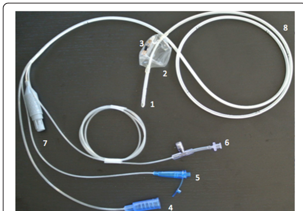
Figure 2 The duodenal photoplethysmographic probe. The duodenal feeding tube with the photoplethysmographic probe. (1) Enteral feeding tube tip for post-pyloric nutrition. (2) Inflatable balloon. (3) Photoplethysmographic sensor. (4) Oro- or nasojejunal feeding line. (5) Aspiration line. (6) Line dedicated to inflate and deflate the balloon and to measure intra-abdominal pressure. (7) Connection line to the sensor. (8) Aspiration hole.
