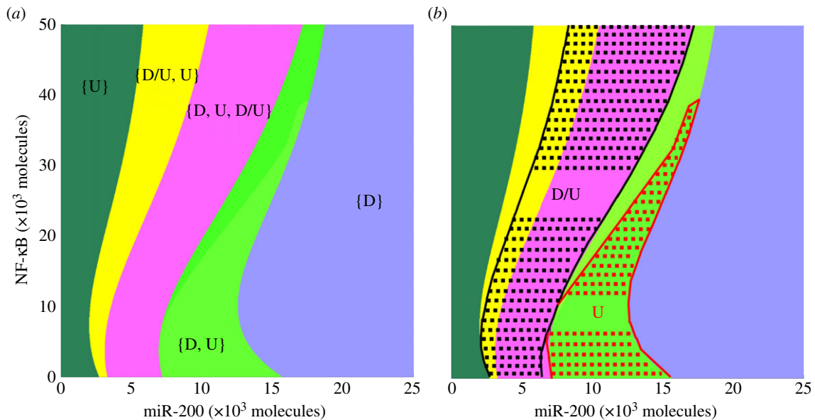
Figure 5. Cells in hybrid E/M state are highly likely to be stem-like. (a) Phase-space diagram of the response of LIN28/let-7 circuit to miR-200 and NF- \kappa B. Each phase corresponds to a different combination of coexisting phenotypes and is denoted by a different colour. For example, in phase \{D\} , cells are in D state; and cells in phase \{D, U, D/U\} can adopt any of the three states—D, U or D/U. (b) Mapped regions for likelihood of stemness, as defined by a range of intermediate OCT4 levels (relative levels = 0.25–0.65). Cells in D/U state in the entire \{D, U, D/U\} phase and part of the \{D/U, U\} phase (as marked with black dotted lines, and bound by black solid lines in yellow region, and black solid lines at the boundary of pink and light green region) have high likelihood of stemness. In addition, cells in the U state are likely to be stem-like in a part of the \{D, U\} region (as marked with red dotted lines and bound by red solid lines in light green region, and red solid lines at the boundary of light green and blue region). Cells in both U and D/U states are both likely to be stem-like in the small area at the bottom (bounded with red and black lines) in the \{D, U, D/U\} phase.
