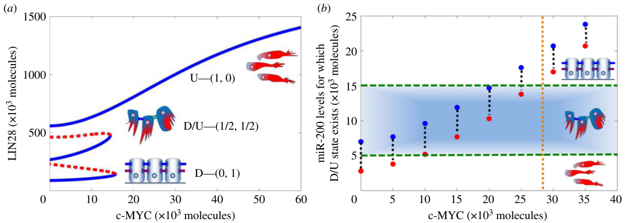
Figure 3. Circuit response to c-MYC and miR-200. (a) Bifurcation diagram showing the dependence of the level of LIN28 on c-MYC when LIN28 is inhibited by constant miR-200 level = 7000 molecules. Blue solid lines indicate stable states, and red dotted lines denote unstable states. Corresponding EMT phenotypes have been indicated for every stable state. (b) Required levels of miR-200 for the D/U—(1/2, 1/2) state to exist for different levels of c-MYC. Red dots show minimum miR-200 levels for which the D/U state can exist, and blue dots are for corresponding maximum values. The area within the green horizontal dashed lines represents the range of miR-200 levels that are associated with the hybrid E/M phenotype (5000–15 000 molecules) [4]. Corresponding phenotypes have been indicated for different states (E, M, E/M) depending on miR-200 levels. Brown vertical dotted line denotes the maximum estimated levels of c-MYC in a cell (approx. 30 000 molecules [37]).
