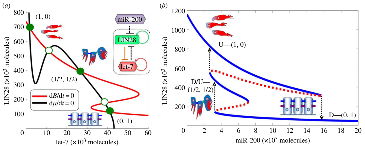
Figure 2. Dynamical behaviour of the LIN28/let-7 circuit. (a) Nullclines and three possible steady states as predicted by the model for fixed miR-200 = 5000 molecules. Red nullcline is for dB/dt = 0 , and black nullcline is for d\mu/dt = 0 . Green solid dots denote possible states (stable fixed points), and green hollow circles denote unstable fixed points (details of stability analysis are given in electronic supplementary material, S6). The states are U—(1, 0) or (high LIN28, low let-7); D—(0, 1) or (low LIN28, high let-7); and D/U—(1/2, 1/2) or (medium LIN28, medium let-7). (b) Bifurcation of LIN28 protein levels in response to inhibition by miR-200. It illustrates the possible coexistence of three states between epithelial (high miR-200 levels) and mesenchymal (low miR-200 levels). Note that for the parameters used in this figure ( c\text{-MYC} = 0 and \text{NF-}\kappa\text{B} = 0 ), D/U state exists for miR-200 levels from 3000 to 7000 molecules, levels that are consistent with typical levels of miR-200 corresponding to the E/M phenotype (5000–15 000 molecules [4]). As is shown later, in the presence of NF- \kappa B, the range of existence of the D/U state can increase from 4000 to 12 000 miR-200 molecules. Starting from the E phenotype, at bottom right part of the blue curve, and decreasing miR-200 levels, the circuit undergoes a transition from the D—(0, 1) state into the D/U—(1/2, 1/2) state. Further decrease in miR-200 to levels that correspond to M phenotype leads to a transition from the D/U state into the U state. Starting from U state and increasing miR-200 levels, the circuit directly undergoes a transition into the D state at miR-200 level that corresponds to the E phenotype.
