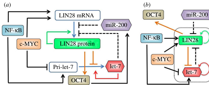
Figure 1. The regulatory network coupling EMT and stemness. (a) Novel modes of regulation in the LIN28/let-7 circuit. LIN28 promotes its own translation (green solid line), and inhibits let-7 processing (orange solid line); let-7 promotes its own processing (red solid line) and inhibits LIN28 translation (black dashed line). NF- \kappa B activates both LIN28 and let-7, whereas c-MYC activates LIN28 and inhibits let-7. miR-200 inhibits LIN28, that translationally activates OCT4 (orange solid arrow) that activates miR-200. (b) Effective circuit showing the LIN28/let-7 double negative feedback loop that receives external input signals from miR-200, c-MYC and NF- \kappa B; and has OCT4 as the output. The activation of miR-200 by OCT4 has not been considered in our current framework. A blue solid line shows conversion of one species to another, a solid black arrow shows transcriptional activation, a solid black bar denotes transcriptional repression, and a black dashed line shows microRNA-mediated translational repression.
