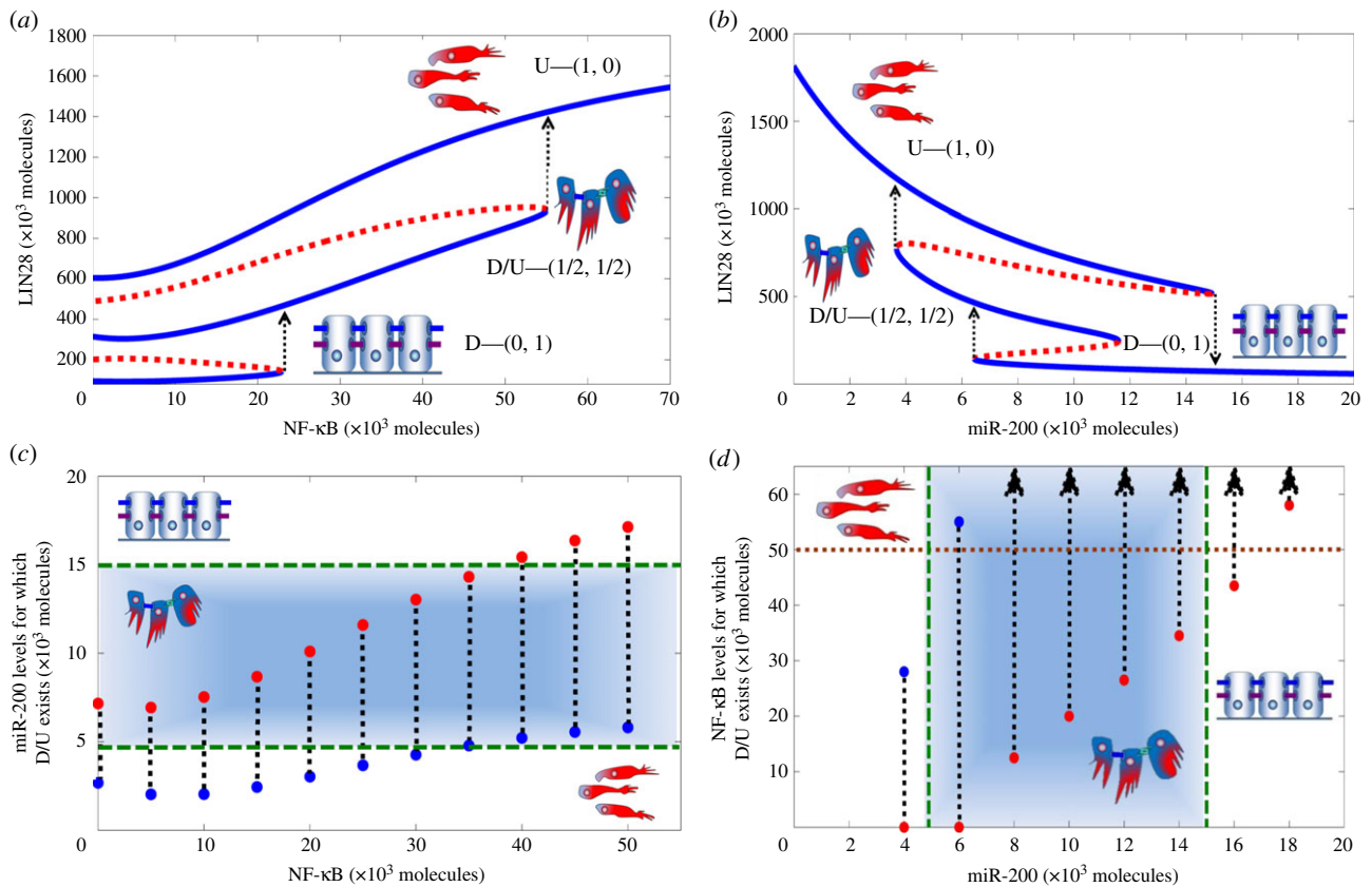
Figure 4. Circuit response to external signals NF- \kappa B and miR-200. (a) Bifurcation diagram shows the dependence of the level of LIN28 on NF- \kappa B when LIN28 is inhibited by constant miR-200 level = 6000 molecules. (b) Complementary bifurcation diagram showing the dependence of the level of LIN28 on miR-200 when the circuit is driven by constant level of NF- \kappa B = 25 000 molecules. Note that the required levels of miR-200 for the existence of D/U state (4000–12 000 molecules) overlap well with the levels of miR-200 for the existence of E/M phenotype (5000–15 000 molecules) [4]. Blue solid lines indicate stable states, and red dotted lines denote unstable states. Corresponding phenotypes (E, M, E/M) have been indicated for every stable state. (c) Range of miR-200 levels for which the D/U—(1/2, 1/2) state exists, for varying values of NF- \kappa B. Red dots show minimum values of miR-200 for which this state exists, and blue dots for corresponding maximum values. Corresponding phenotypes have been indicated for different states (E, M, E/M) depending on miR-200 levels. (d) Range of NF- \kappa B values for which D/U state exists for different values of miR-200. Red dots are for minimum values of NF- \kappa B for which this state exists, and blue dots are for corresponding maximum values. Arrows denote that the corresponding maximum levels for NF- \kappa B are greater than 60 000 molecules. Brown horizontal dotted line denotes the maximum estimated levels of NF- \kappa B in a cell (50 000 molecules [39]). Areas within the green dashed lines—horizontal in (c) and vertical in (d)—represent miR-200 levels that are associated with the hybrid E/M phenotype.
