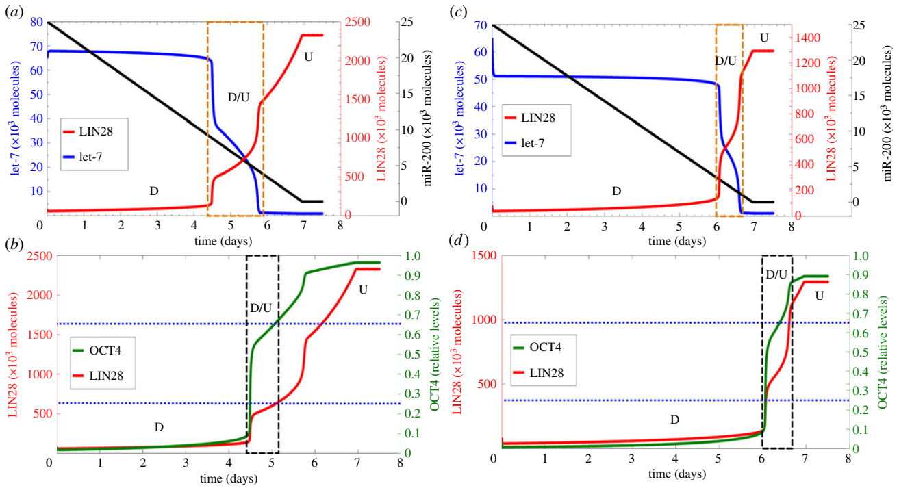
Figure 6. Temporal dynamics of partial and complete epithelial–hybrid–mesenchymal transition. Panels (a,c) show the temporal evolution of let-7 (blue) and LIN28 (red) for fixed \text{NF-}\kappa\text{B} = 40\,000 molecules and \text{NF-}\kappa\text{B} = 10\,000 molecules, respectively, as miR-200 (black) levels decrease over time. The area in the brown rectangle shows the transition from D state (low LIN28, high let-7) to D/U state (medium LIN28, medium let-7) and then to the U state (low LIN28, high let-7). Panels (b,d) denote temporal evolution of OCT4 (green) corresponding to LIN28 (red) levels for \text{NF-}\kappa\text{B} = 40\,000 molecules and \text{NF-}\kappa\text{B} = 10\,000 molecules, respectively. Horizontal dotted blue lines show the range of OCT4 for stemness, and the black rectangle highlights the corresponding values of LIN28 for which the cells are likely to adopt stemness.
