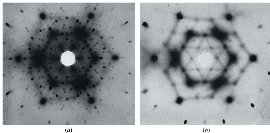
Figure 1 Laue photographs of benzil, C_{14}H_{10}O_2 , adapted from plate 8 of Lonsdale & Smith (1941). The incident beam is approximately along [0001]. (a) Using unfiltered Cu radiation. (b) Using monochromatic Cu K\alpha radiation.
